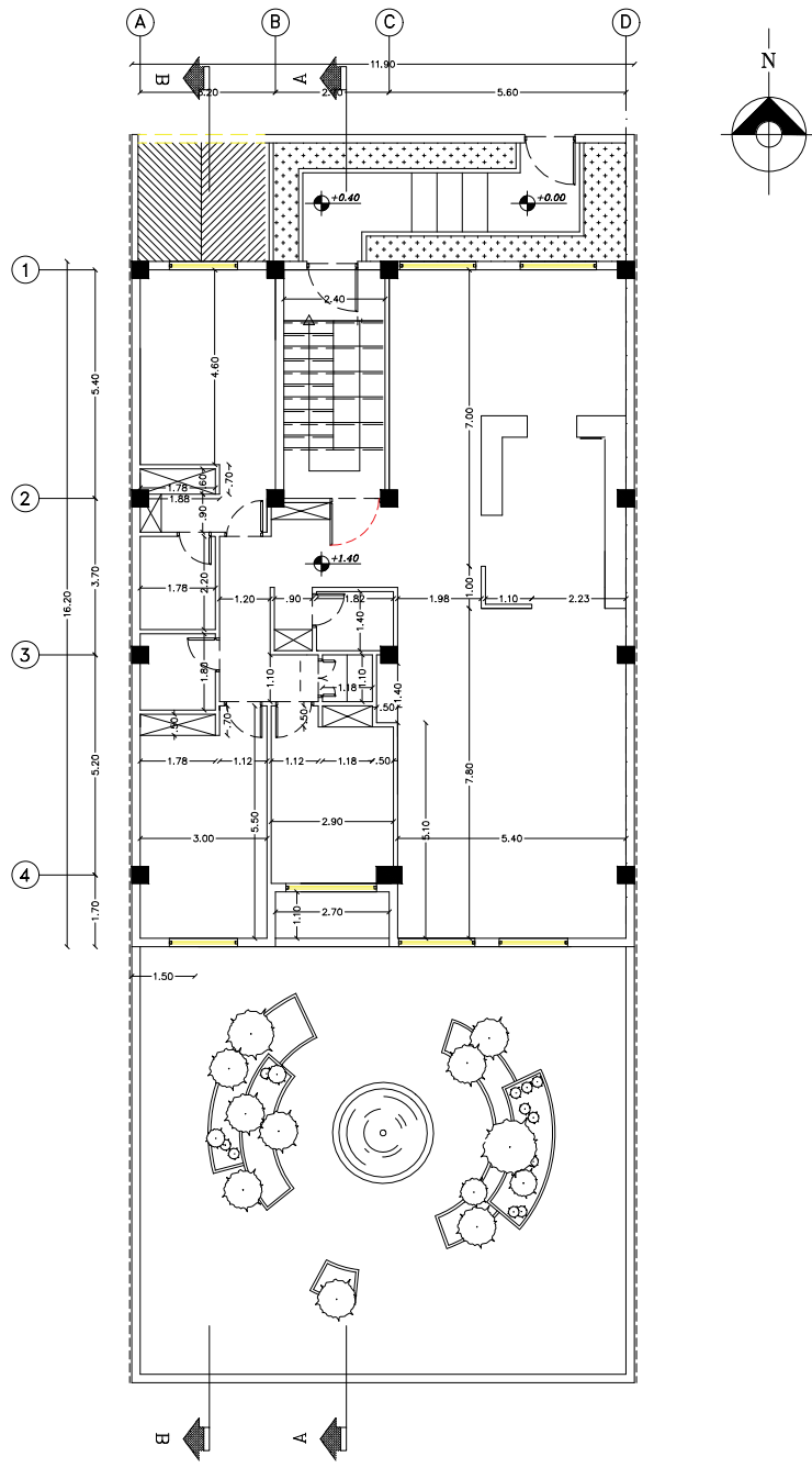
Ground FLOOR PLAN SC: 1/100
