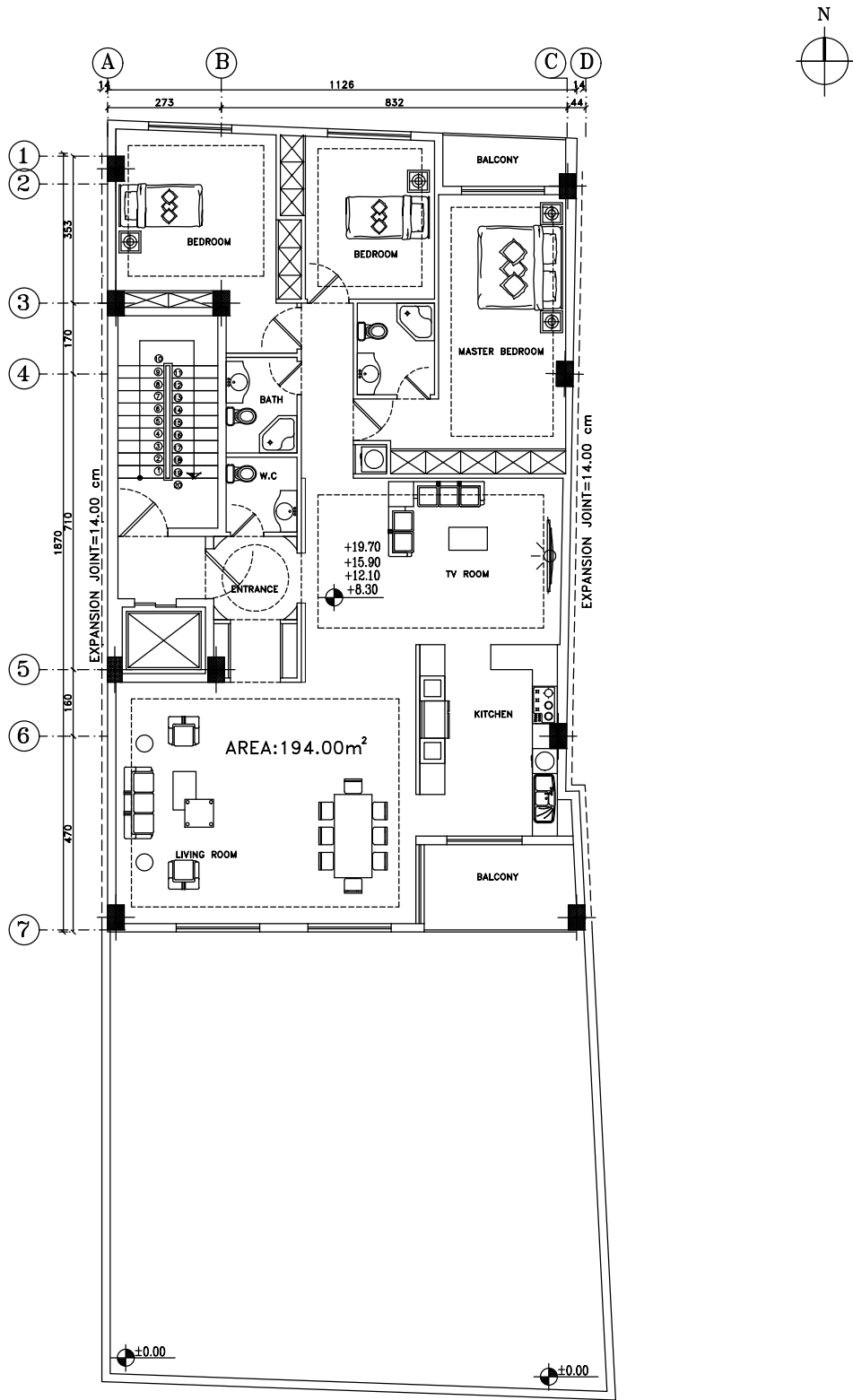
2, 3, 4, 5 FLOOR PLAN
