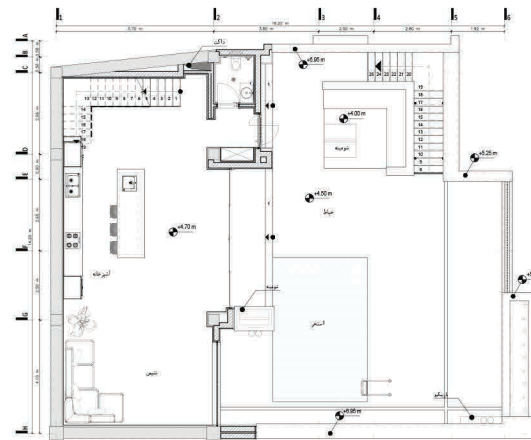
level 02 FIRST floor plan- level: +4.50 SC: 1/75 AREA : 100 M2
