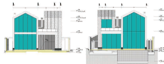
Elavations
