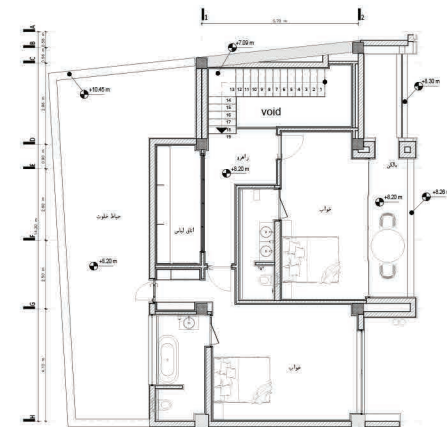
level 03 SECOND floor plan- level: +6.00 SC: 1/75 AREA : 105 M2
