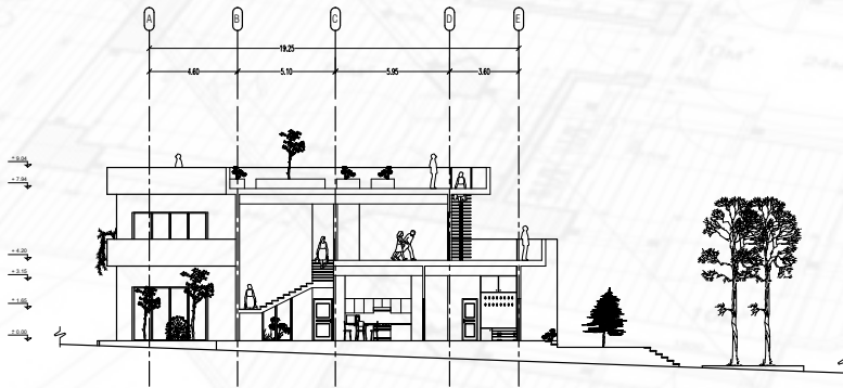
B-B section
