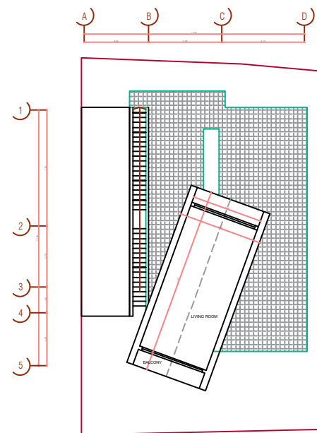
FLOOR DIMENSION PLAN
