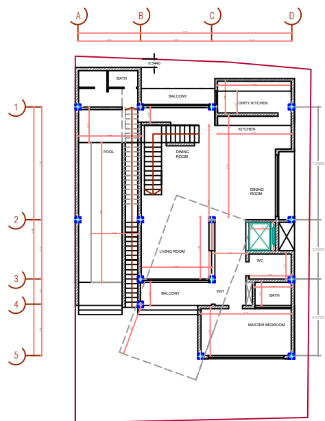
GROUND FLOOR DIMENSION PLAN
