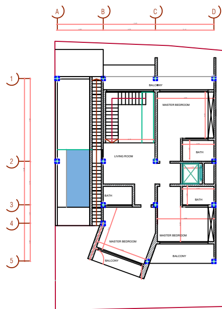
FIRST FLOOR DIMENSION PLAN
