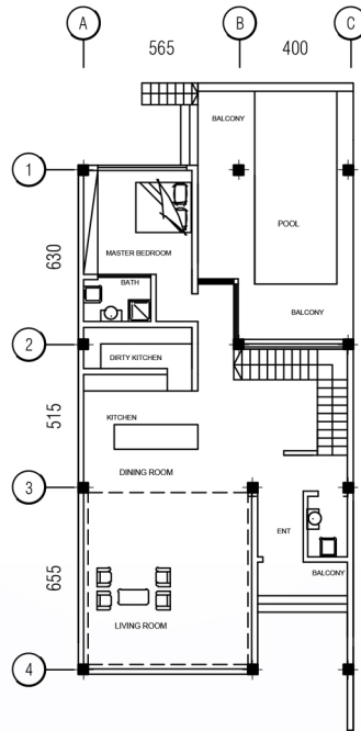
GROUND FLOOR FURNITURE PLAN Sc:1/100 AREA : 135 M2
