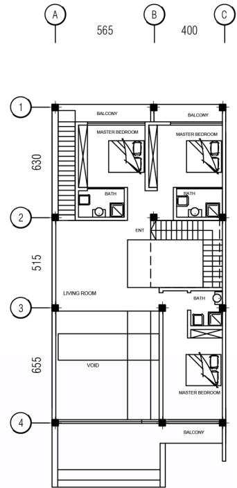
FIRST FLOOR FURNITURE PLAN Sc:1/100 AREA : 183 M2
