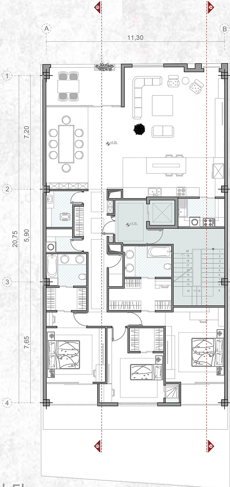
Second Floor
