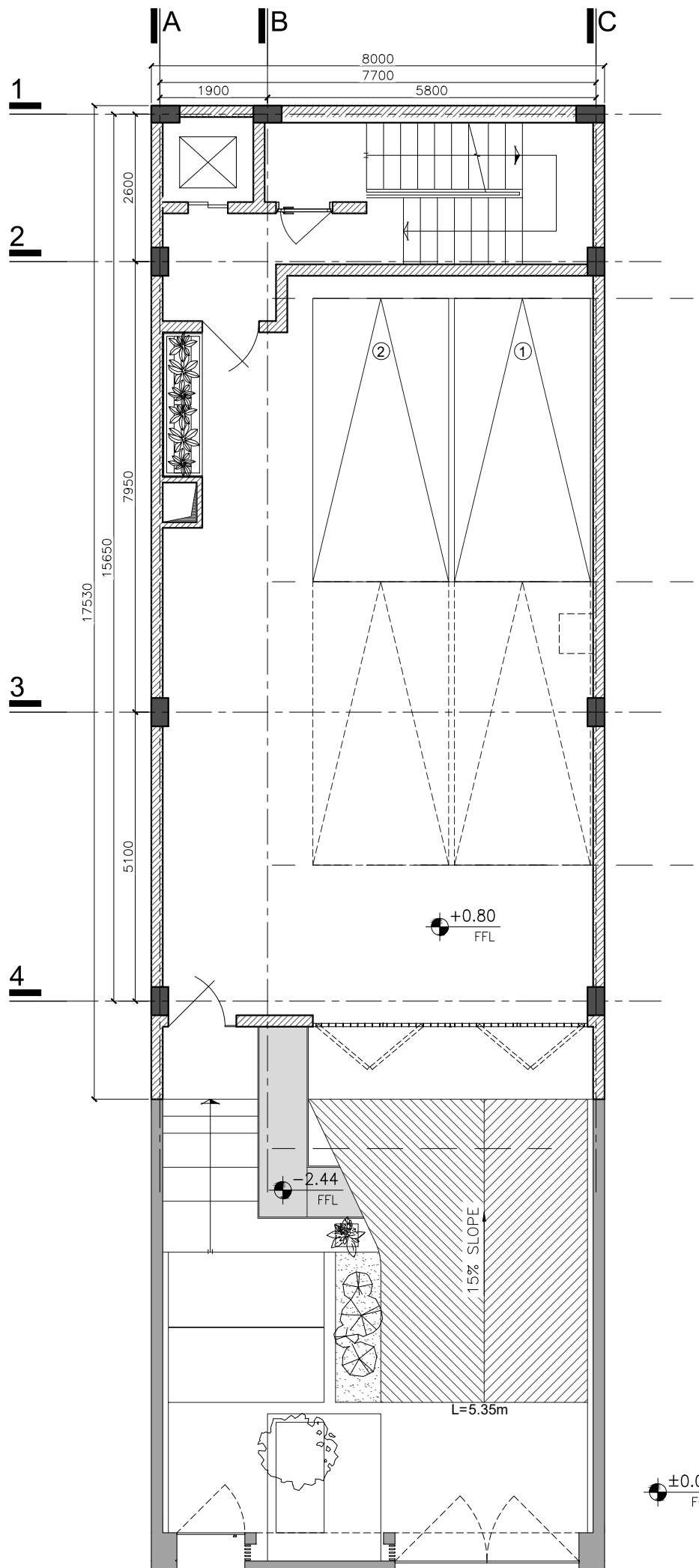
1 GROUND FLOOR PLAN 1:100
