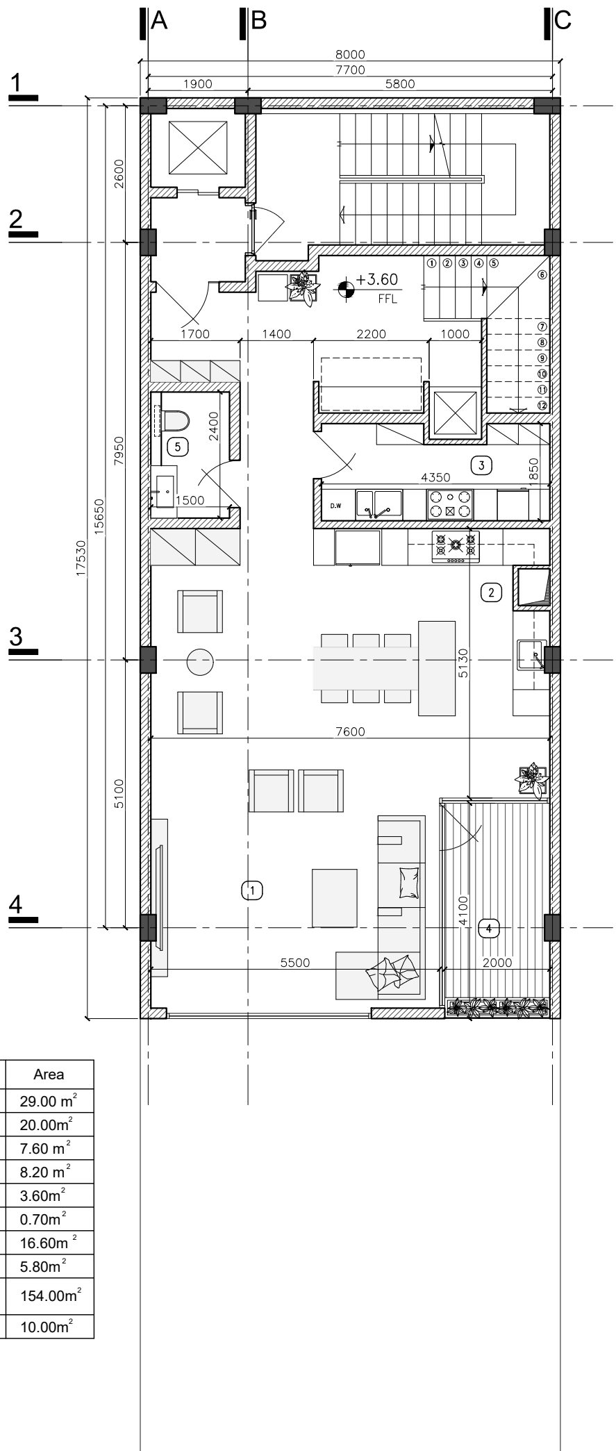
1 FIRST FLOOR PLAN 1:100
