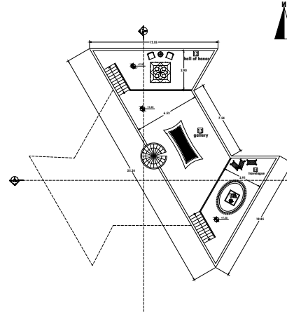
1st floor plan scale: 1:100
