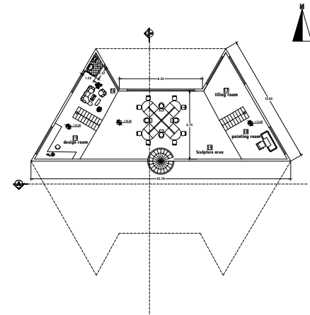
2nd floor plan scale: 1:100
