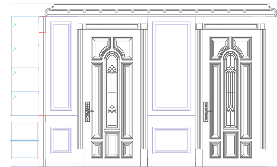
B-B VIEW
