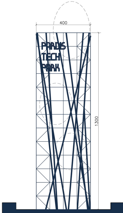
West Elevation
