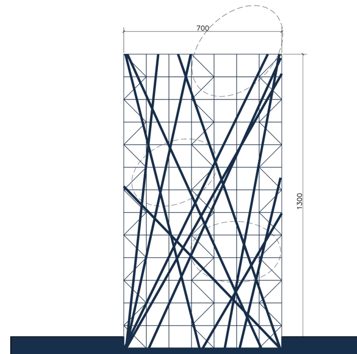
North Elevation
