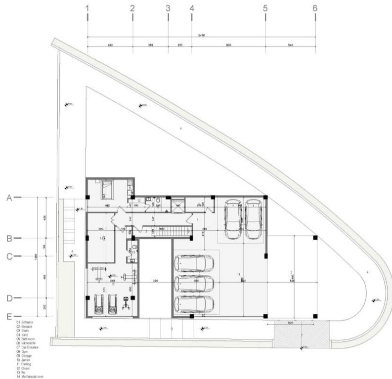
LEVEL GF
