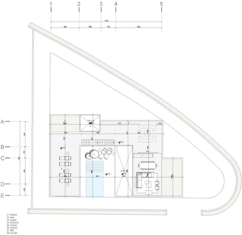
LEVEL ROOF
