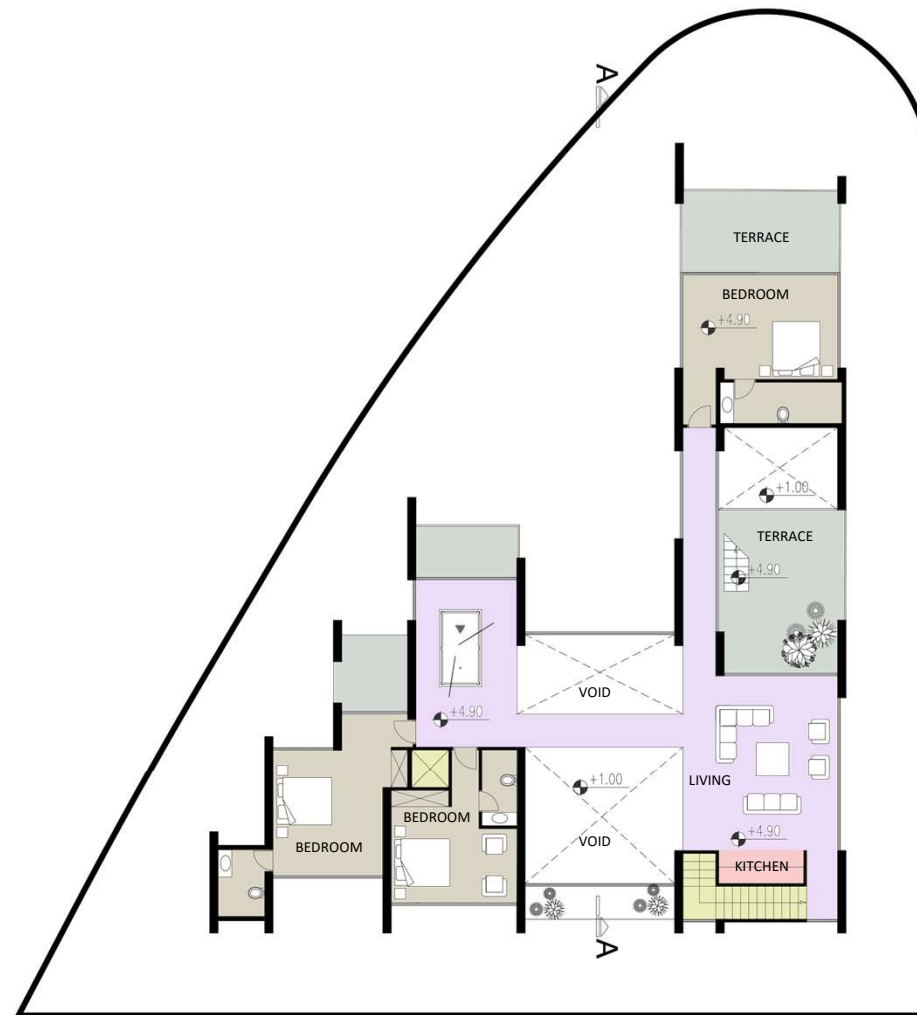
FIRST FLOOR PLAN 242 sqm
