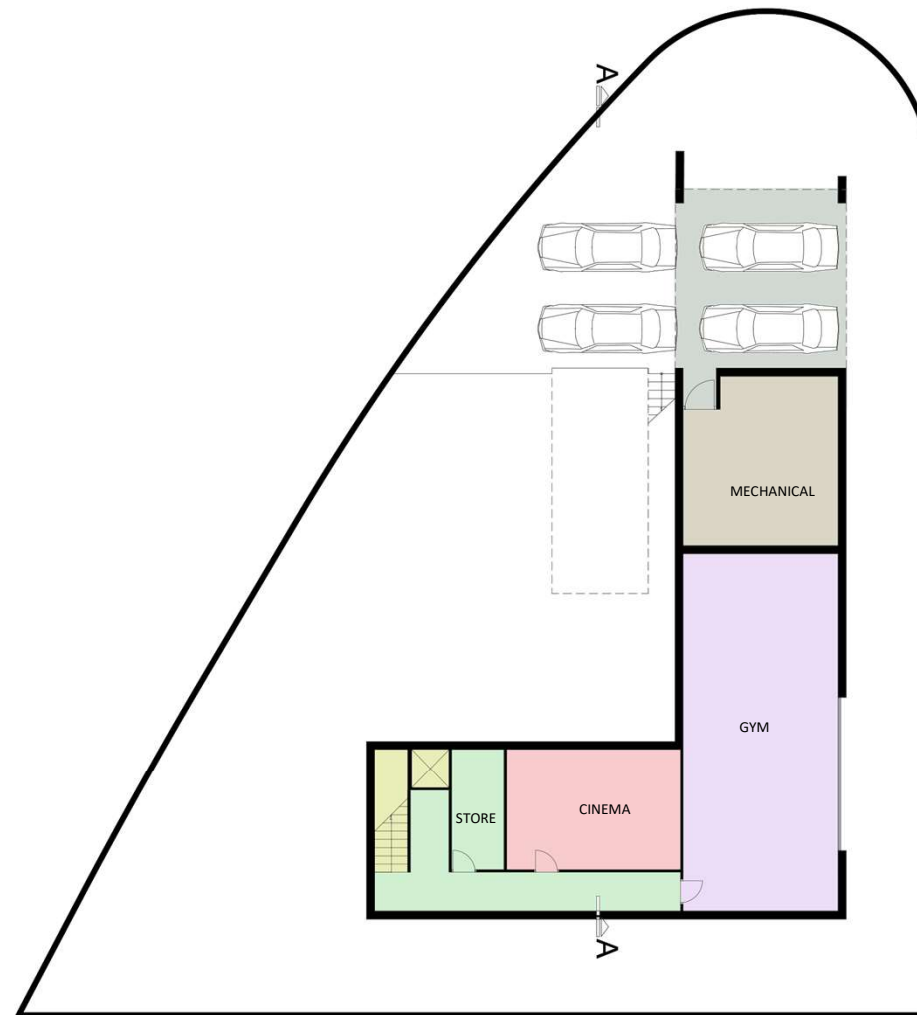
BASEMENT PLAN
