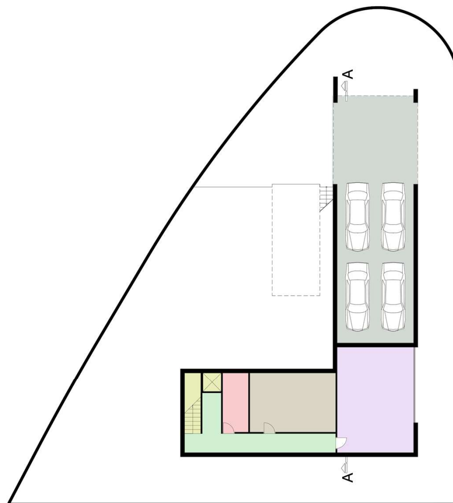
BASEMENT PLAN
