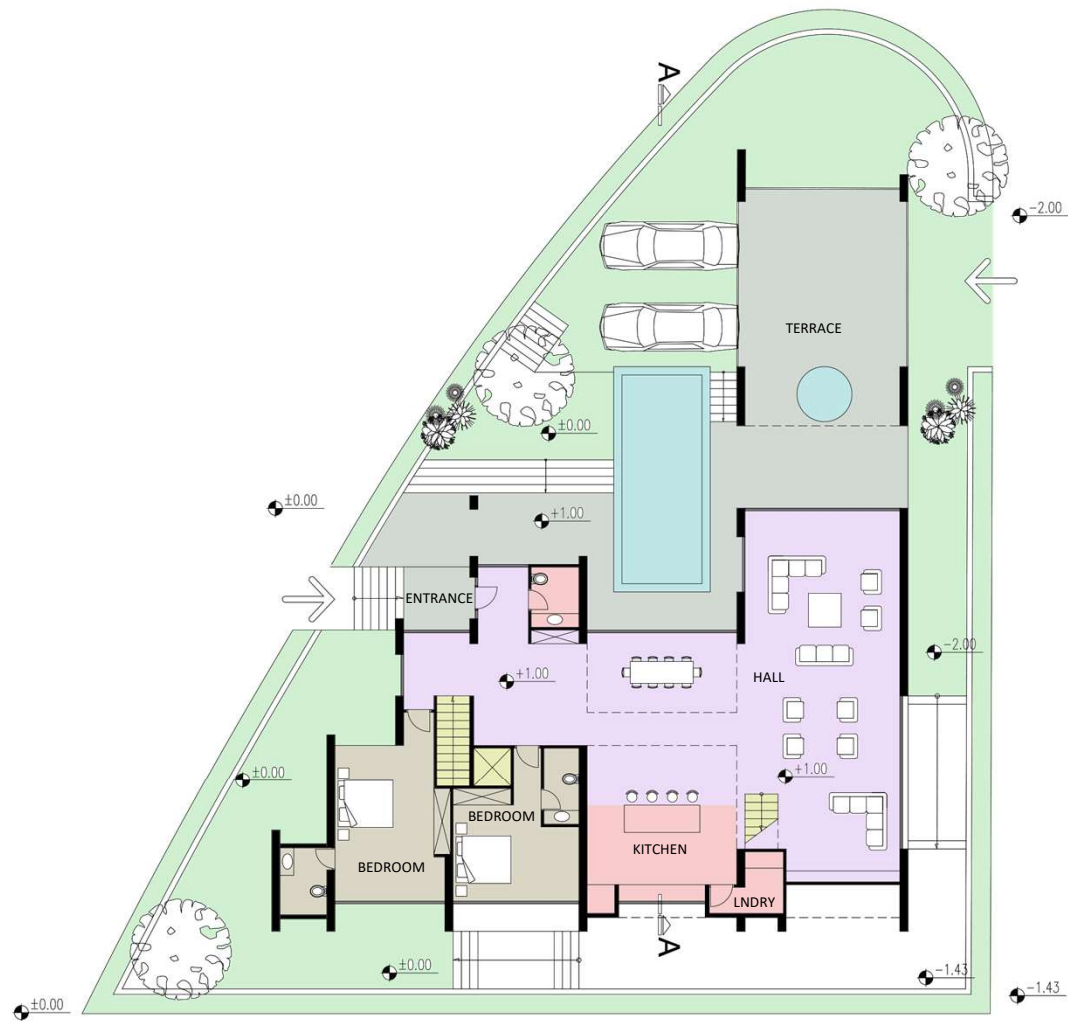
GROUND FLOOR PLAN 241 sqm
