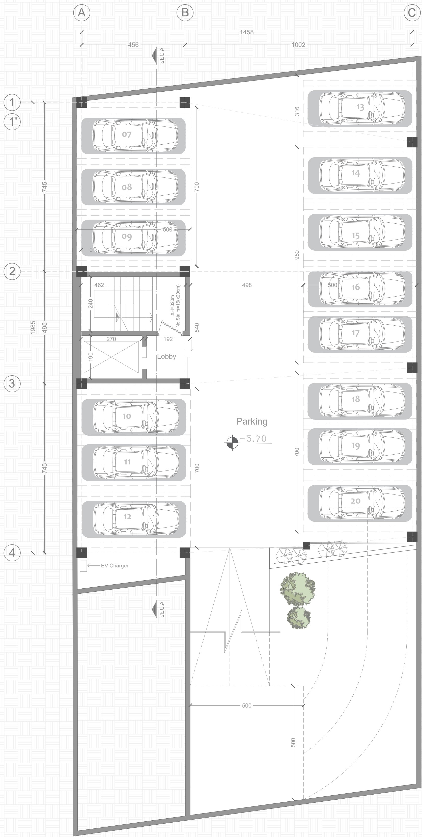
Second Basement_Dimension Plan
