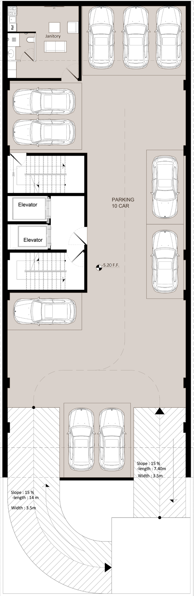
PLAN ALT 1 B2
