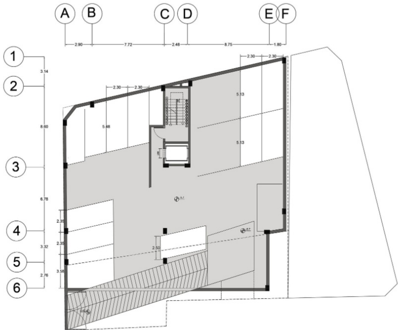
-2 FLOOR PLAN
