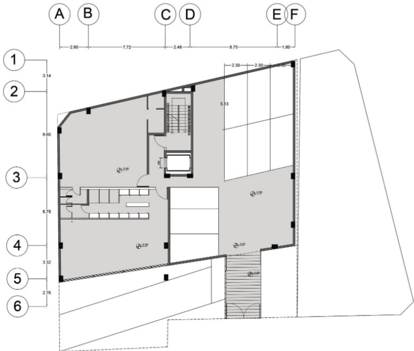
-1 FLOOR PLAN
