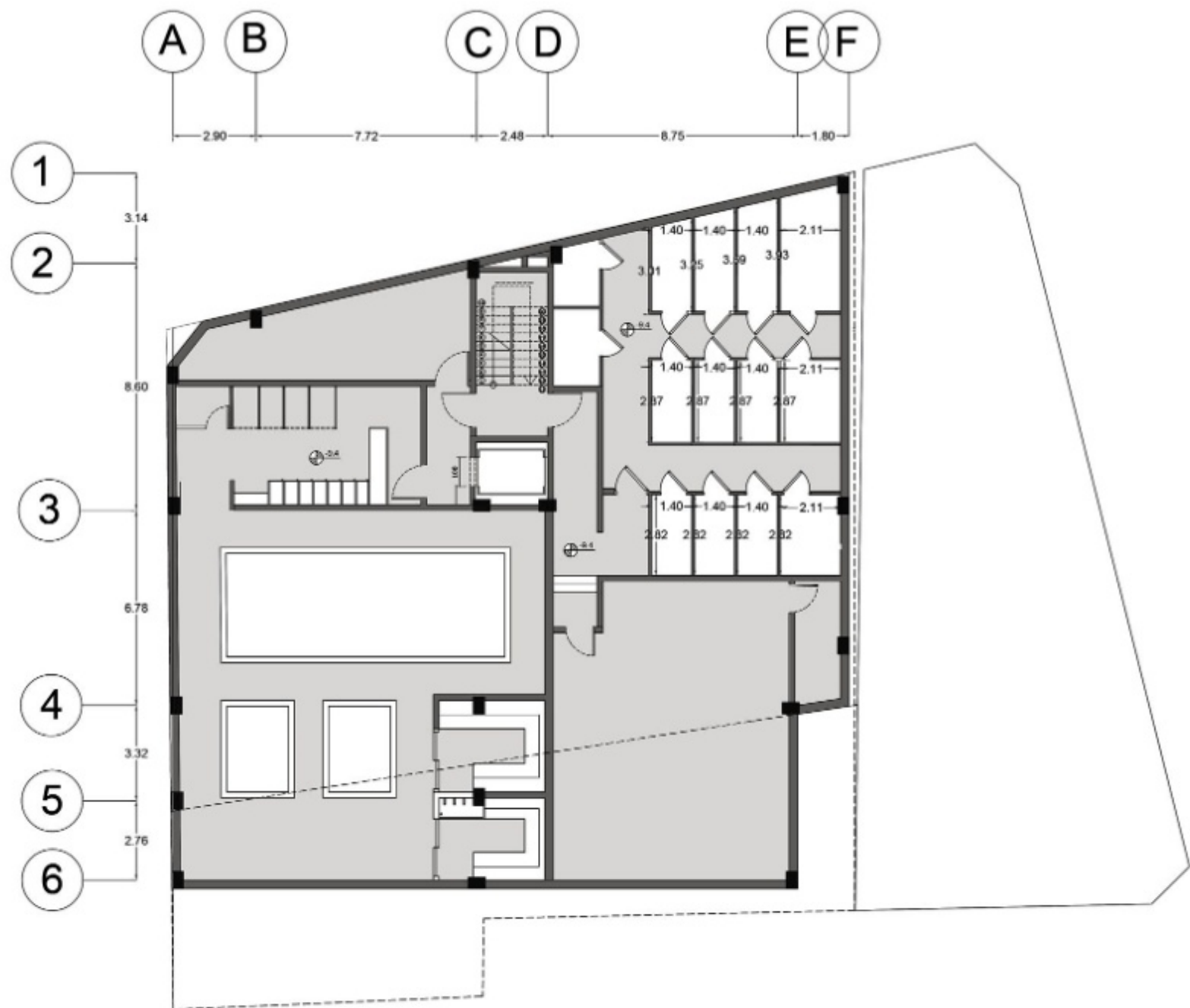
-3 FLOOR PLAN
