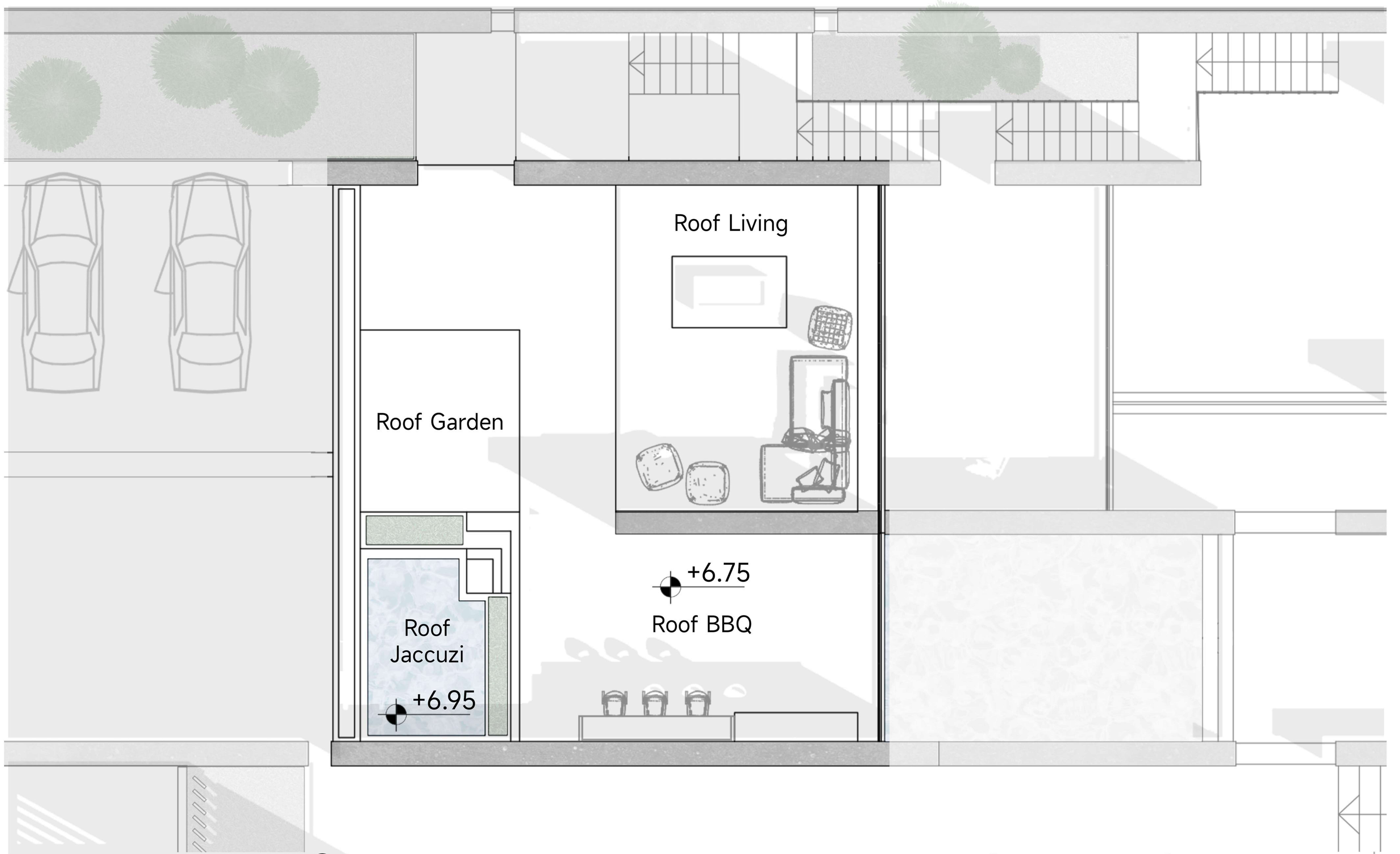
ROOF GARDEN PLAN (⊖)
