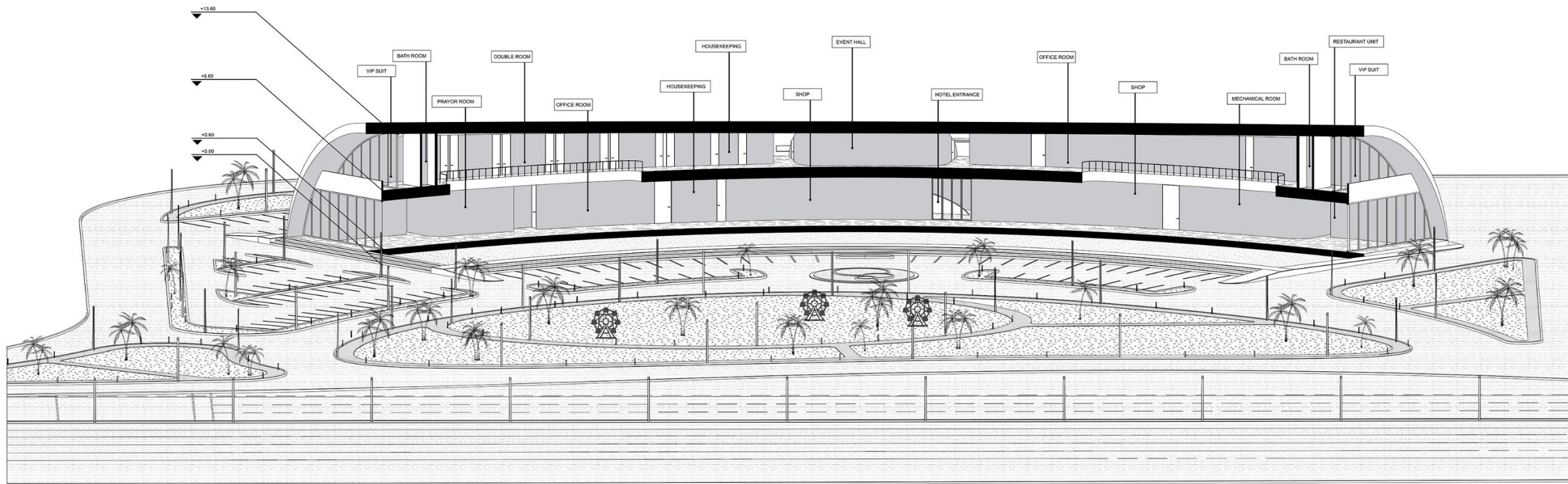
SECTION 3D
