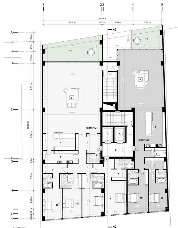
AVIN RESIDENCE-L1,3,5,7,9,11-ALT04
