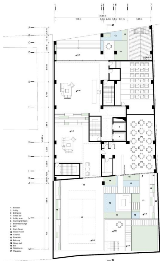
AVIN RESIDENCE-GF-ALT02
