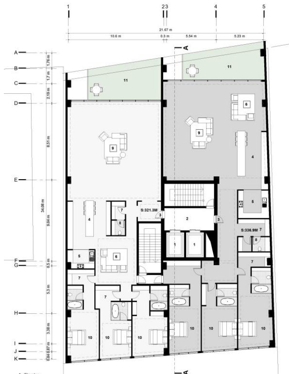
AVIN RESIDENCE-L1,3,5,7,9,11-ALT01
