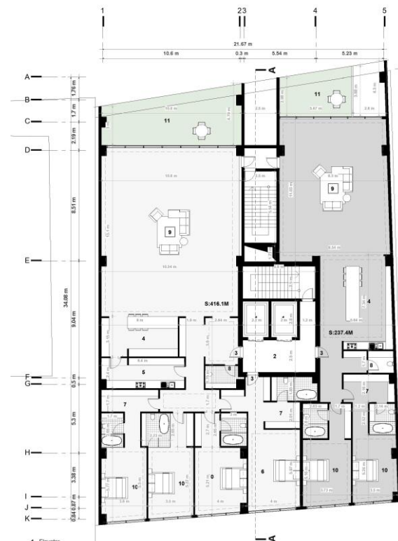
AVIN RESIDENCE-L2,4,6,8,10-ALT04
