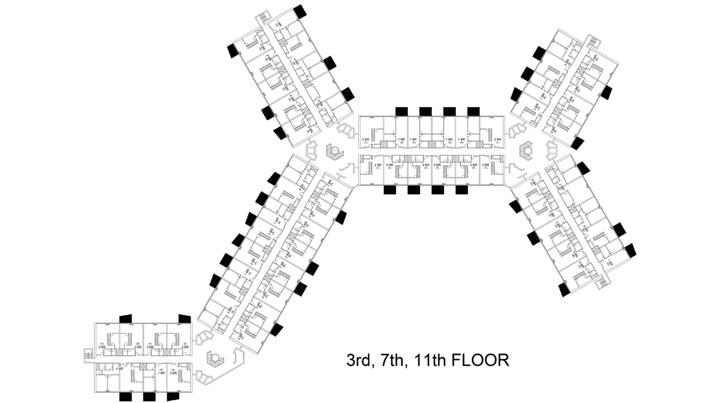
EKBATAN '75 Phase 2, Block 16 Floor Plans (with balconies)
