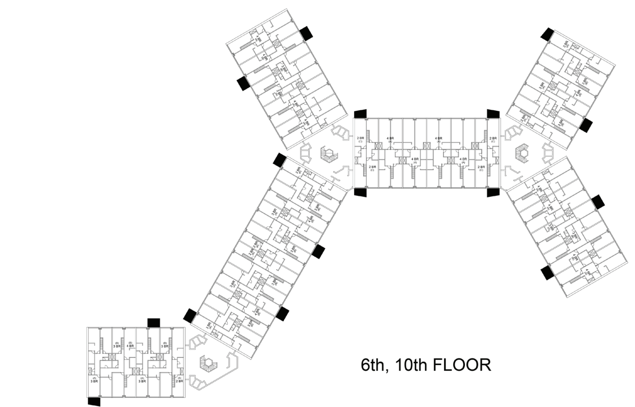
EKBATAN '75 Phase 2, Block 16 Floor Plans (with balconies)
