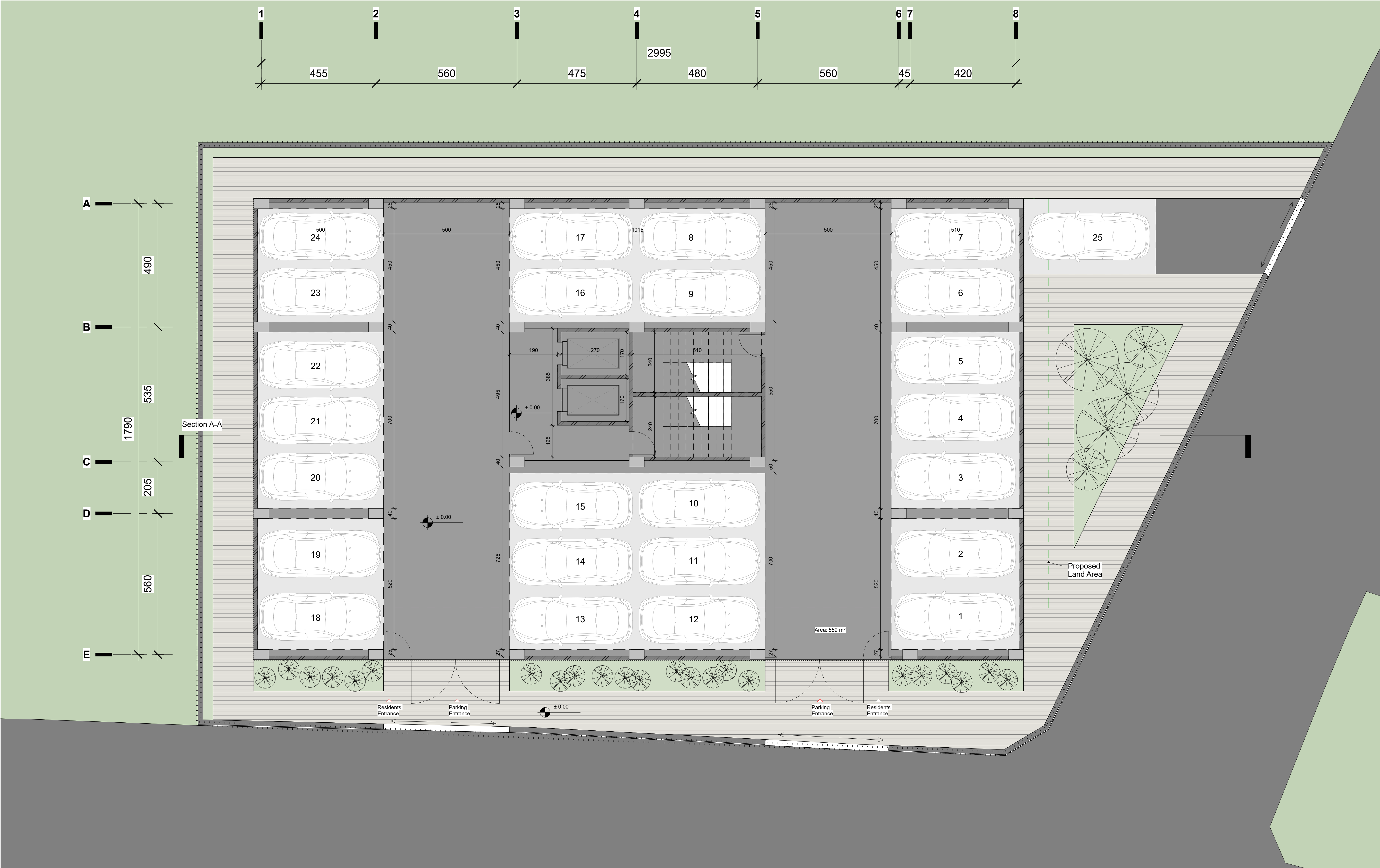
Ground Floor Dimension Plan
