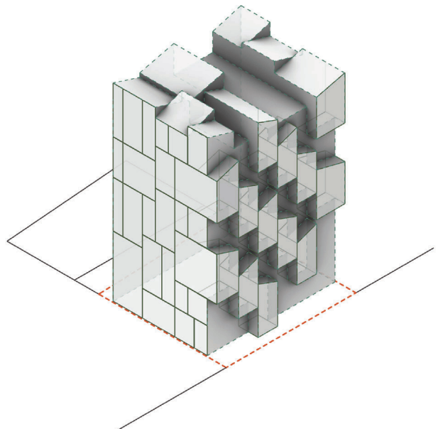
5. Designing the Third Facade in Alignment with the Main Facade Lines
