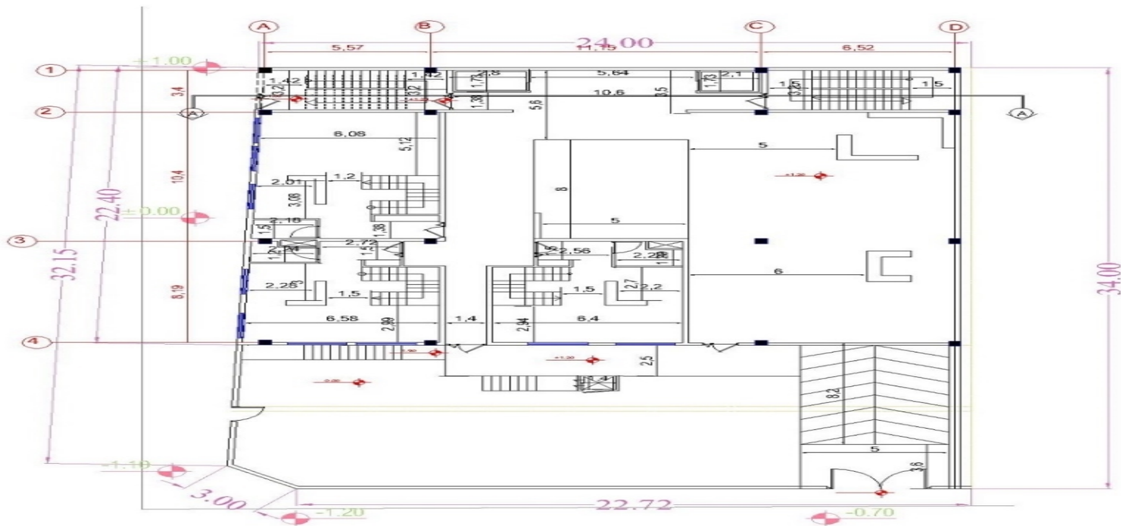
Measurement Plan Ground Floor
