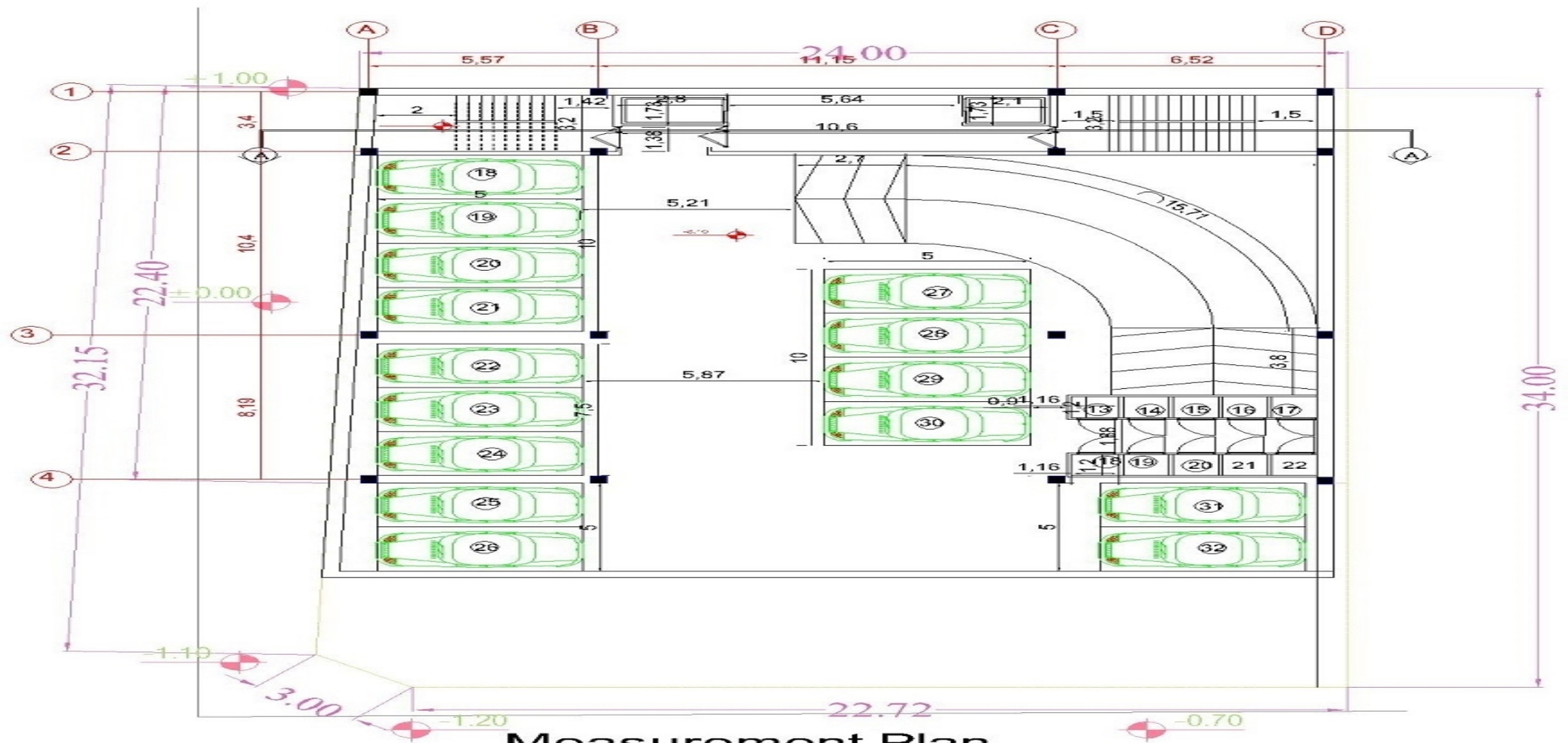
Measurement Plan Negative Floor Three
