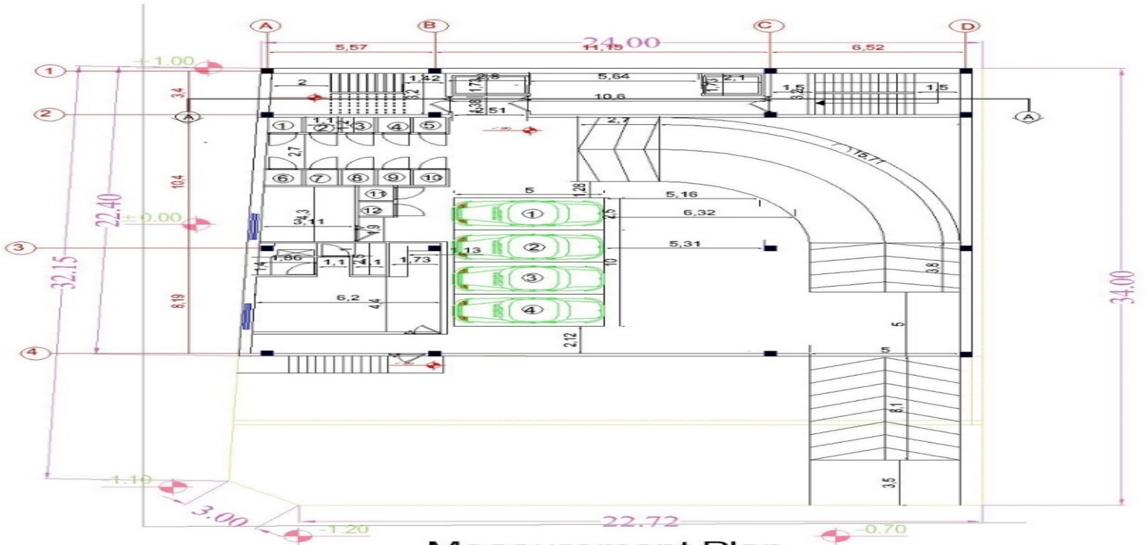
Measurement Plan Negative Floor One
