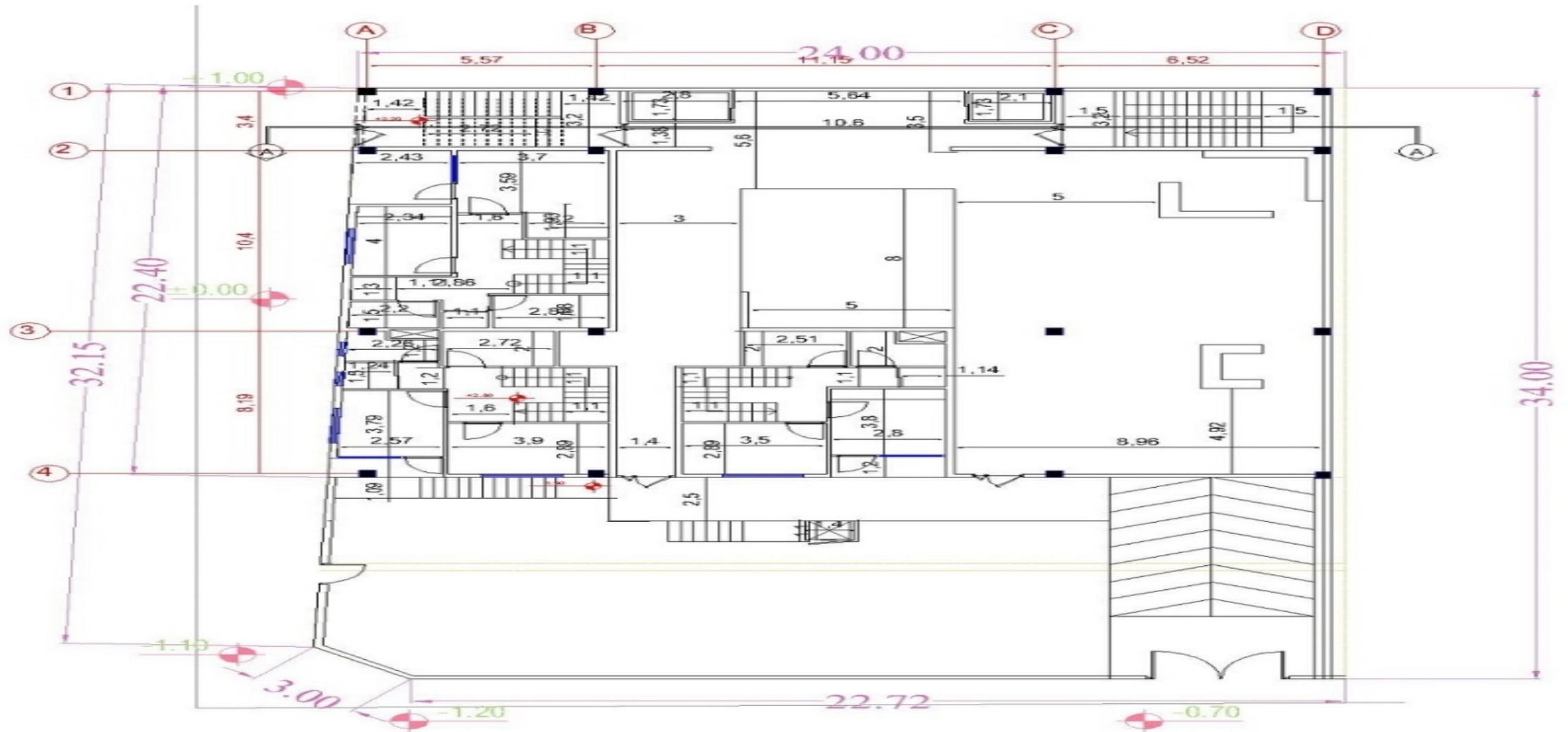
Duplex Floor
