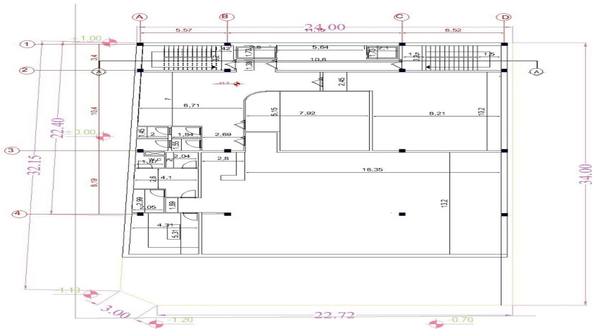
Measurement Plan Negative Floor Four
