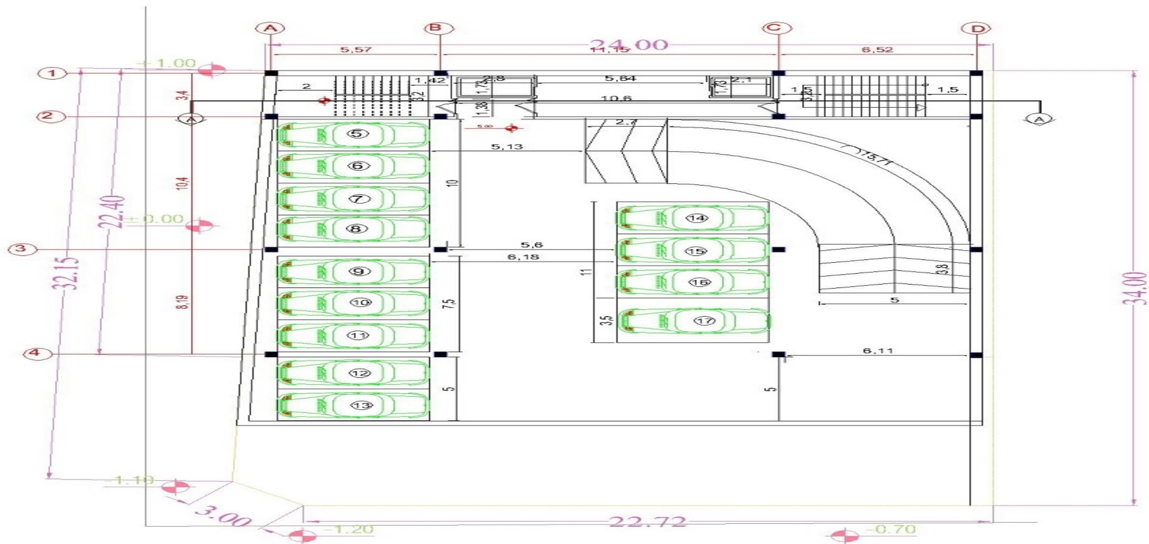
Measurement Plan Negative Floor Two
