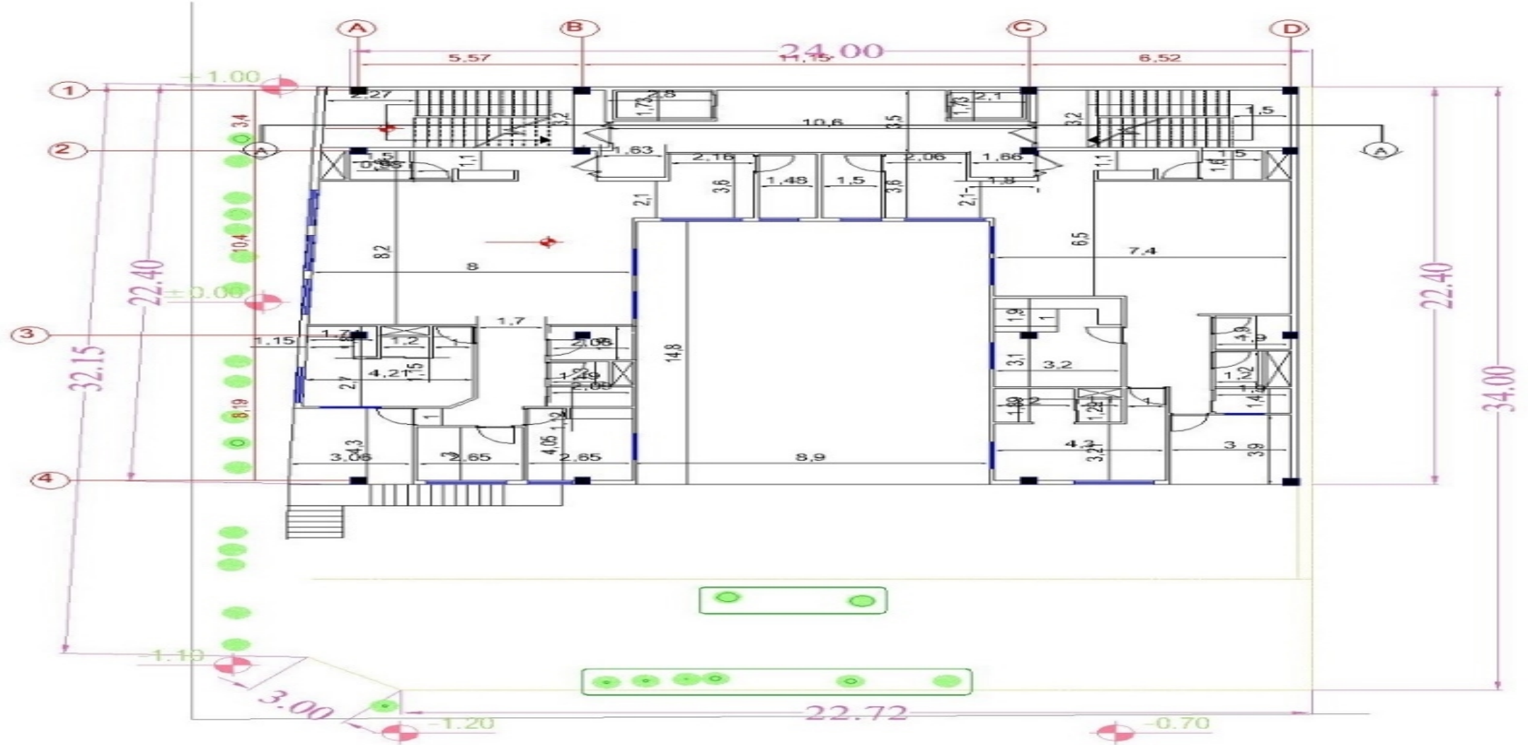
Measurement Plan Floor Type
