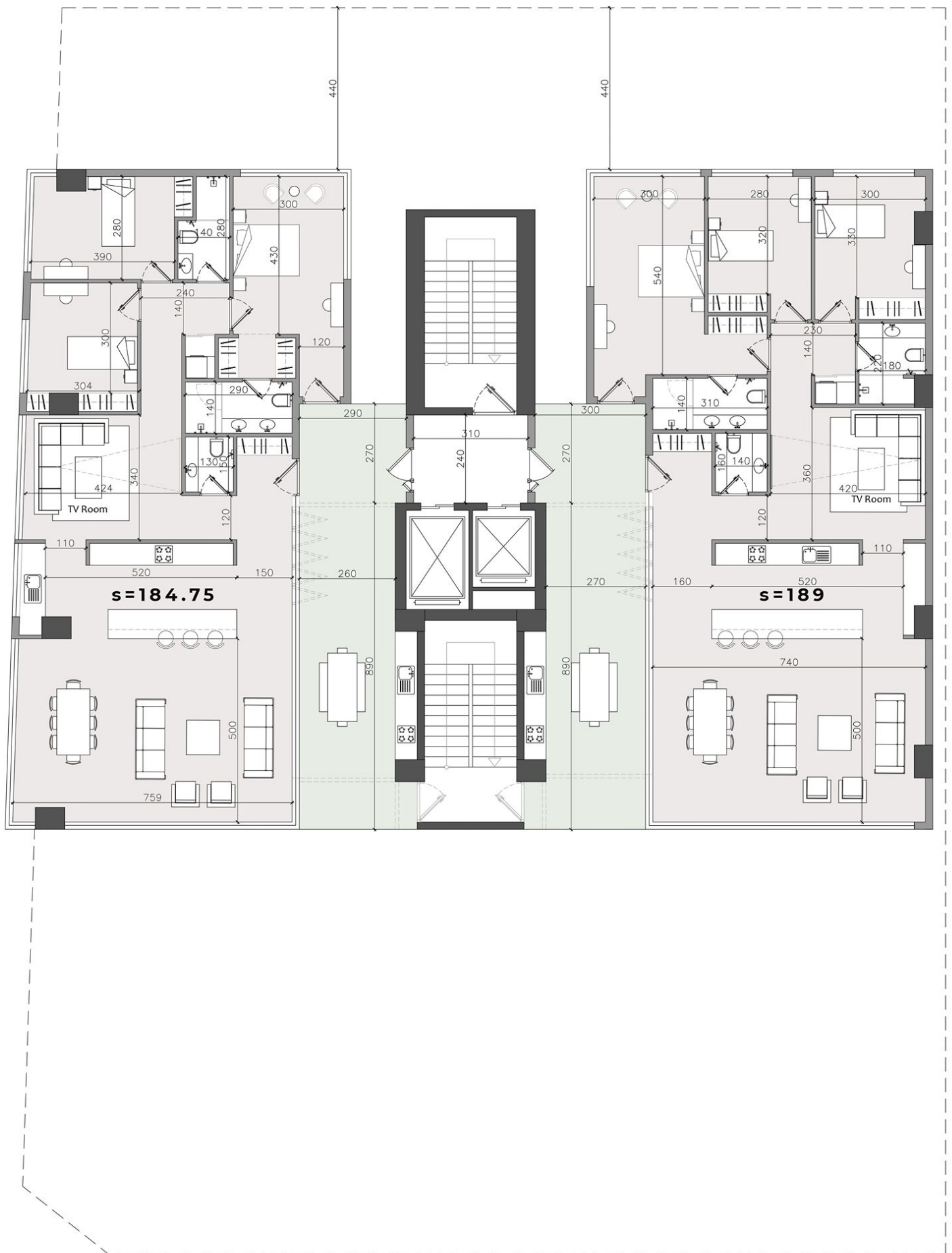
Floor plan
