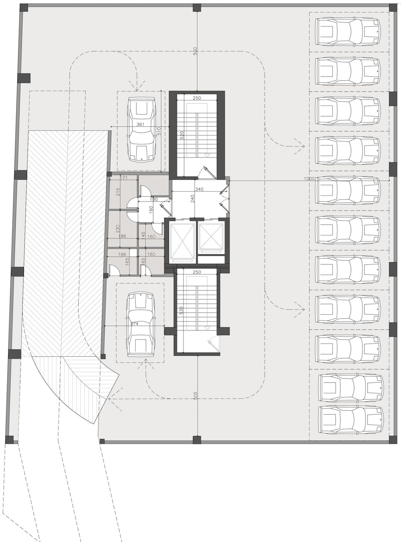
Basement 2
