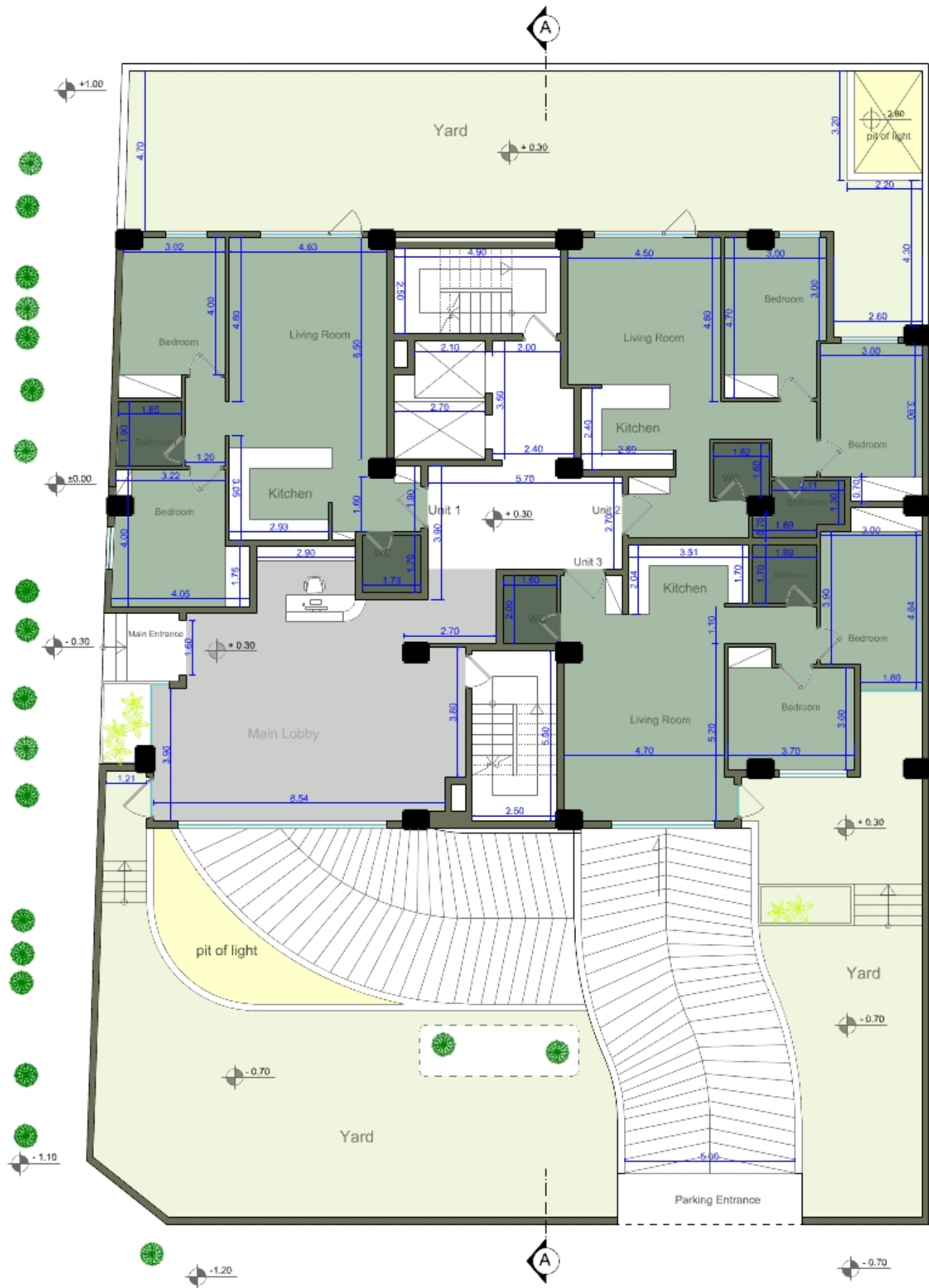
Dimension plan ....(GF)
