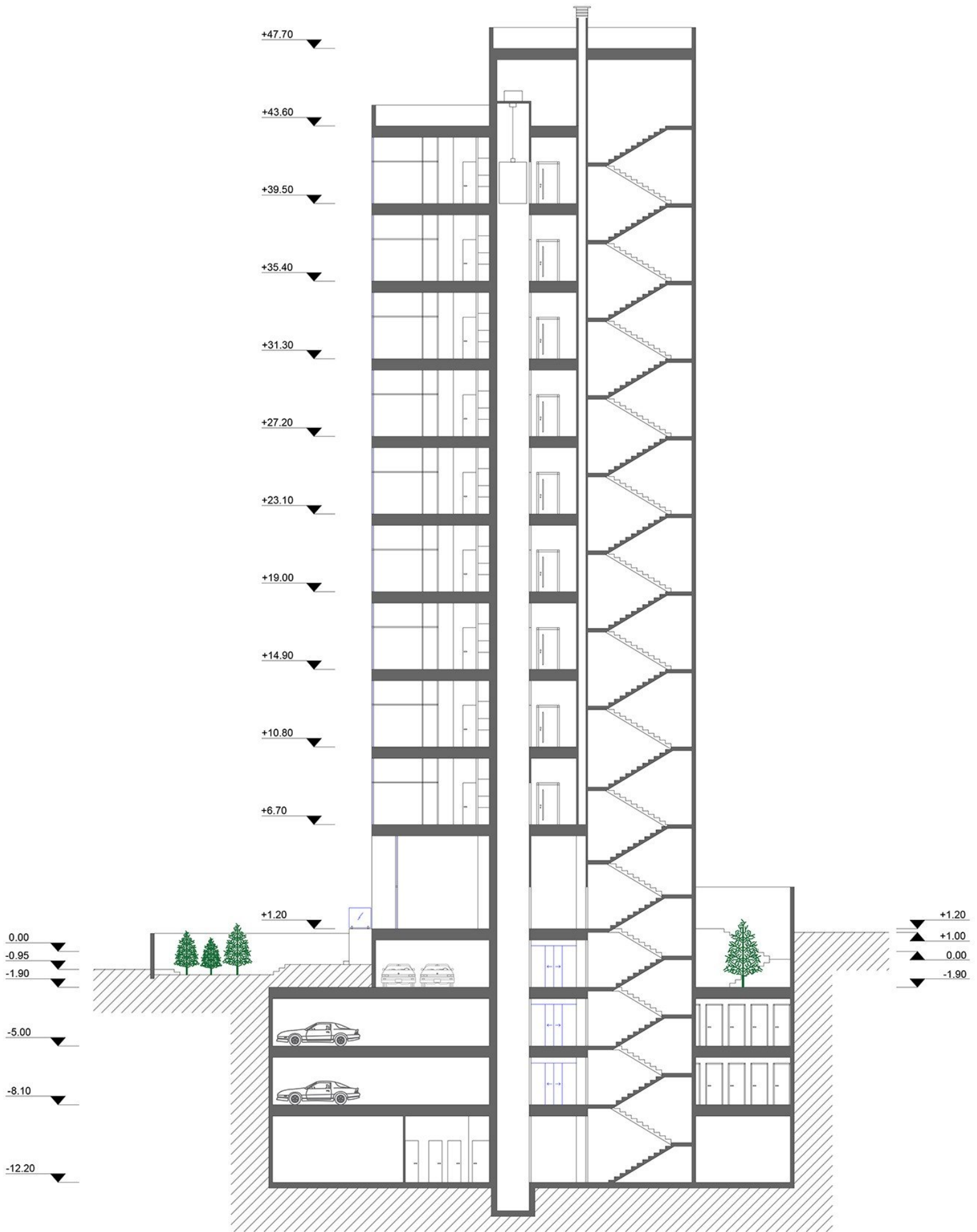
ROZ apartment section A-A
