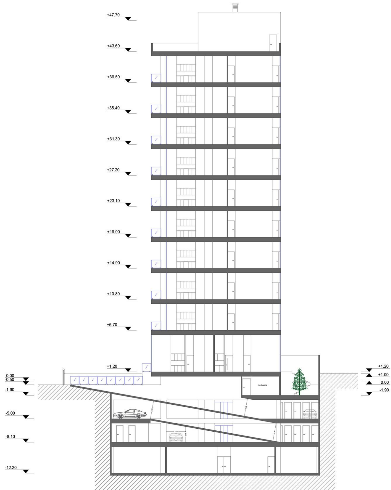
ROZ apartment section B-B
