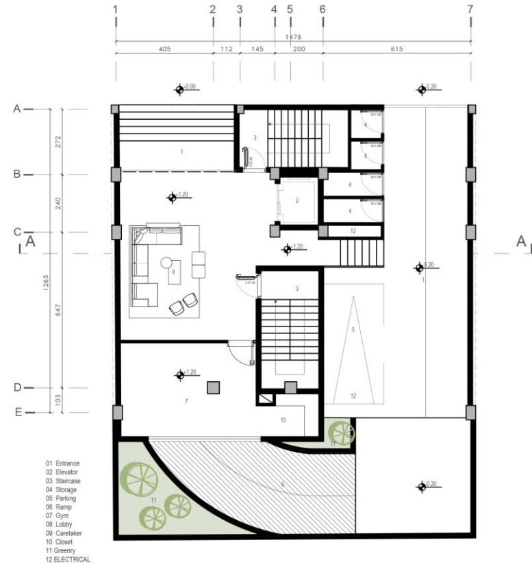
LEVEL GF FURNITURE PLAN
