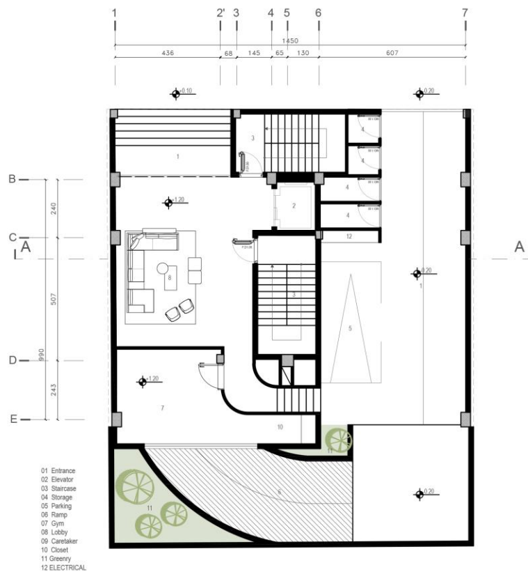
LEVEL GF - ALT05 FURNITURE PLAN
