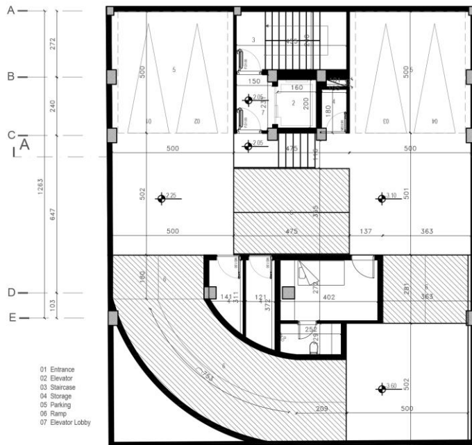
LEVEL -01 DIMENSION PLAN
