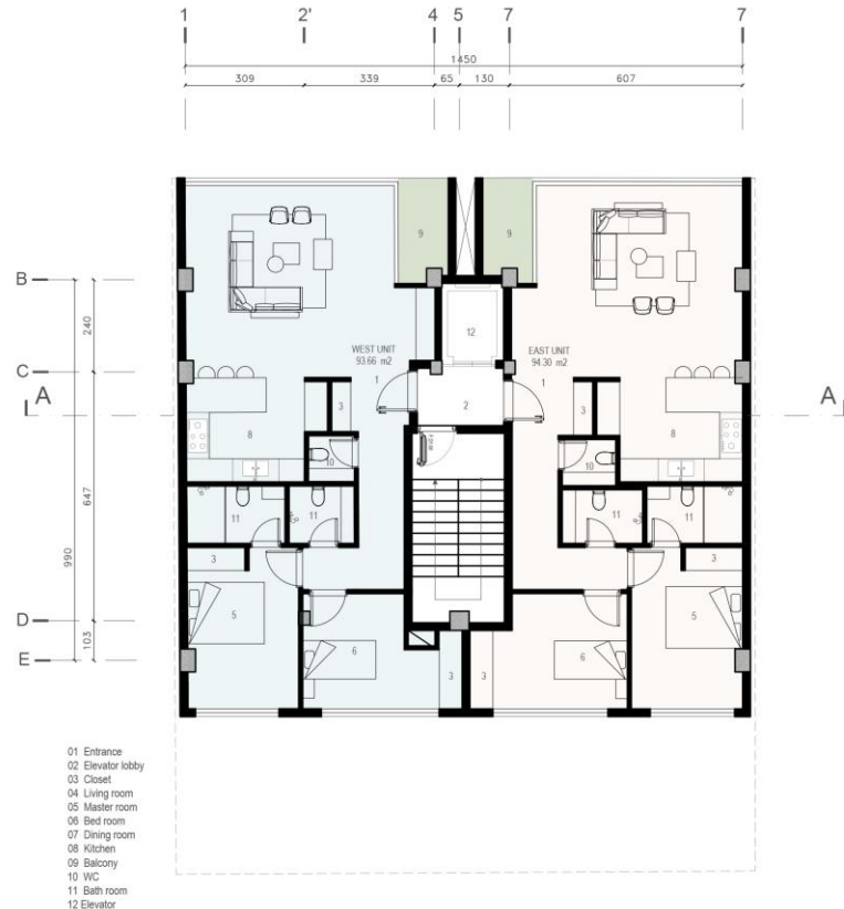
LEVEL TYPICAL - ALT04 FURNITURE PLAN
