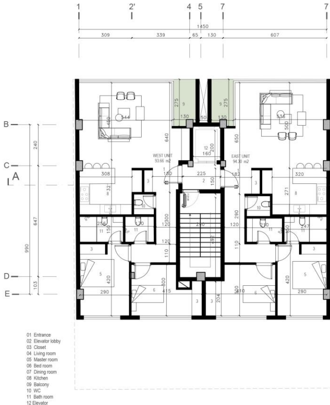
LEVEL TYPICAL - ALT04 DIMENSION PLAN
