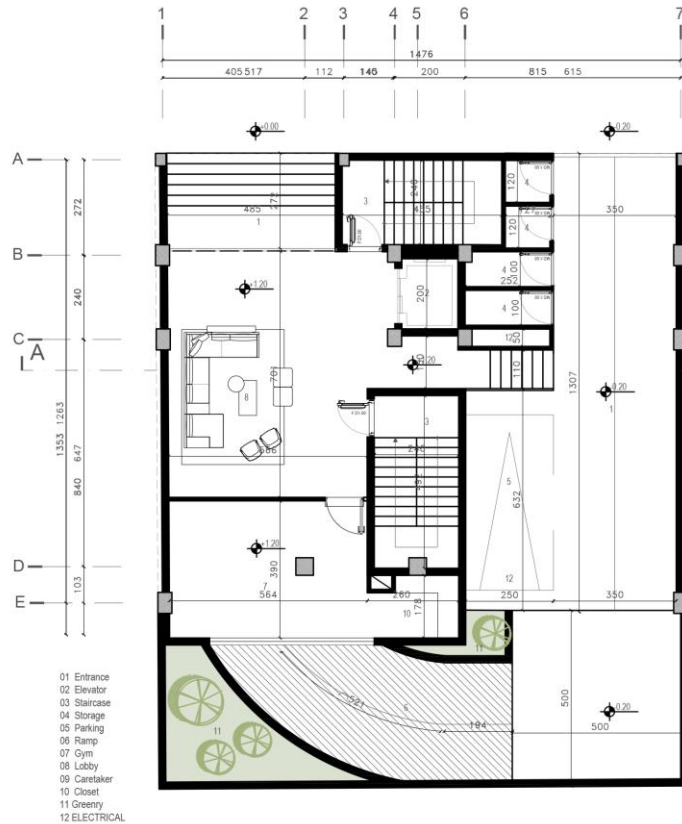
LEVEL GF DIMENSION PLAN
