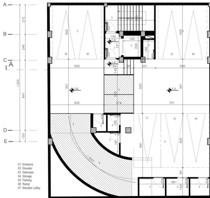
LEVEL -02 DIMENSION PLAN
