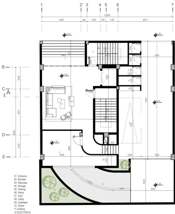
LEVEL GF - ALT05 DIMENSION PLAN
