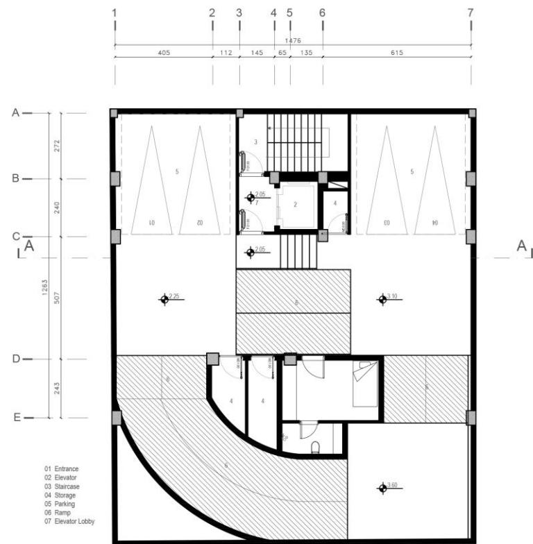
LEVEL -01 - ALT05 FURNITURE PLAN
