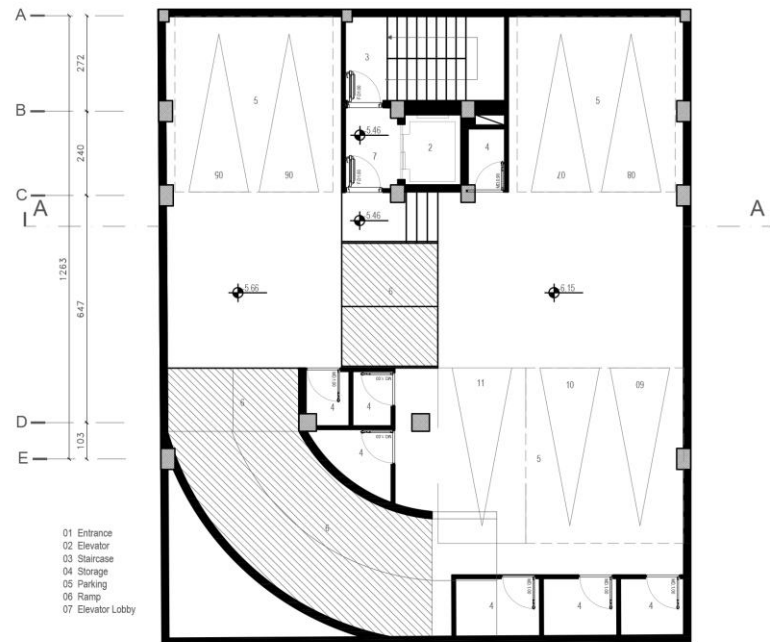
LEVEL -02 FURNITURE PLAN
