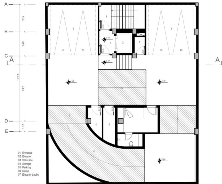
LEVEL -01 FURNITURE PLAN
