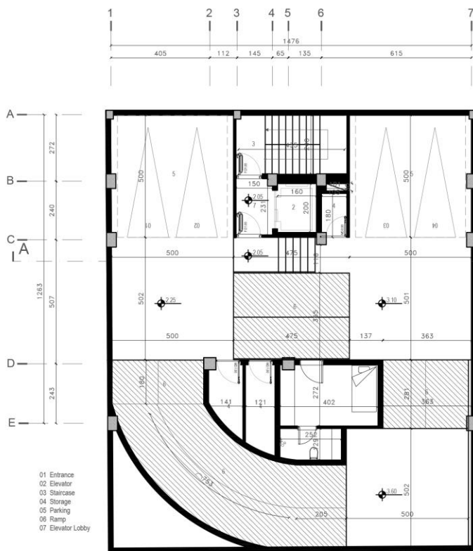
LEVEL -01 - ALT05 DIMENSION PLAN
