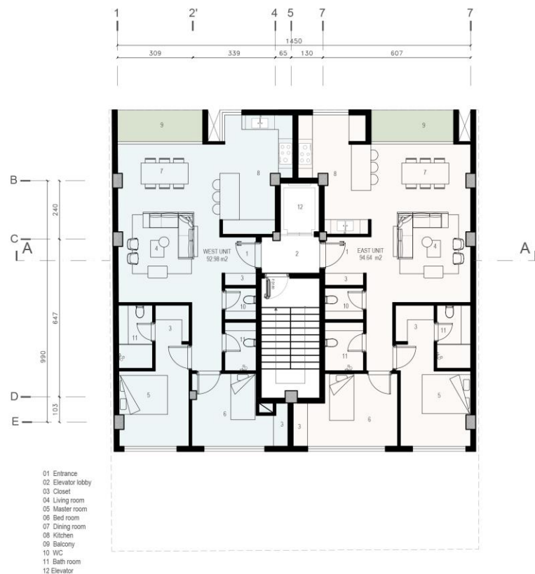
LEVEL ,02,04,06 - ALT03 FURNITURE PLAN
