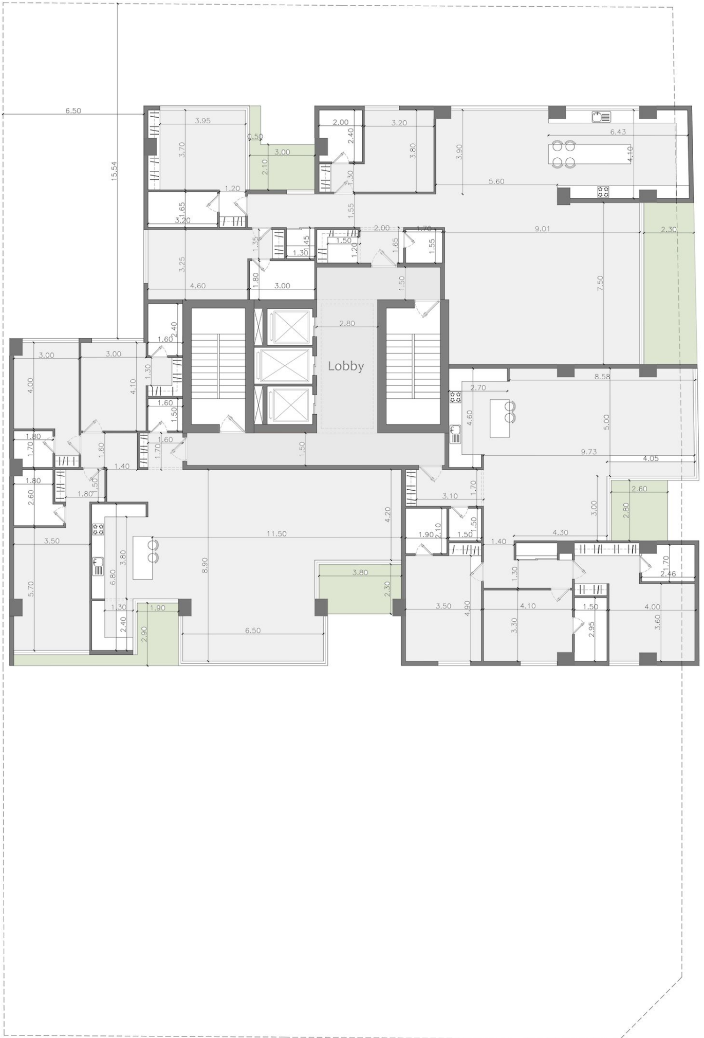
Floor 10_Dimension
