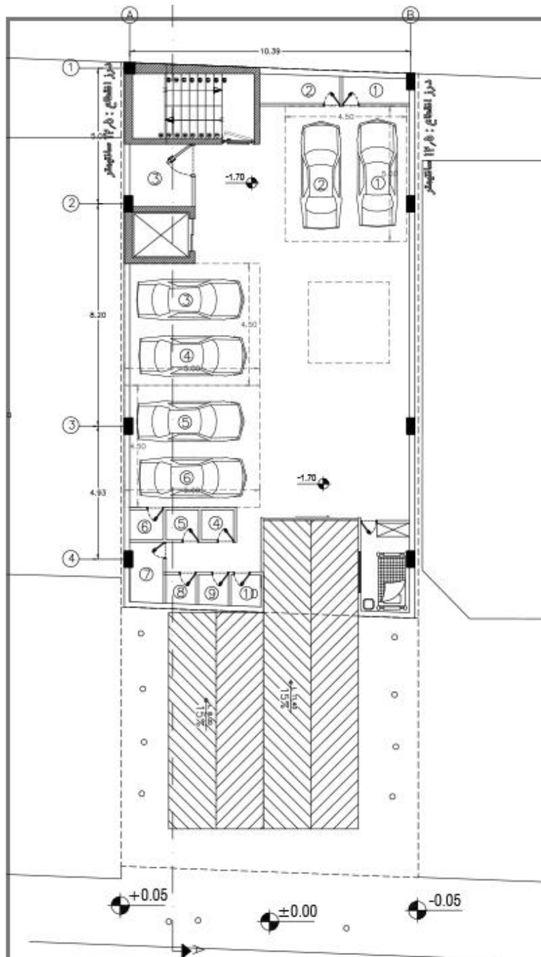
Basement Plane
