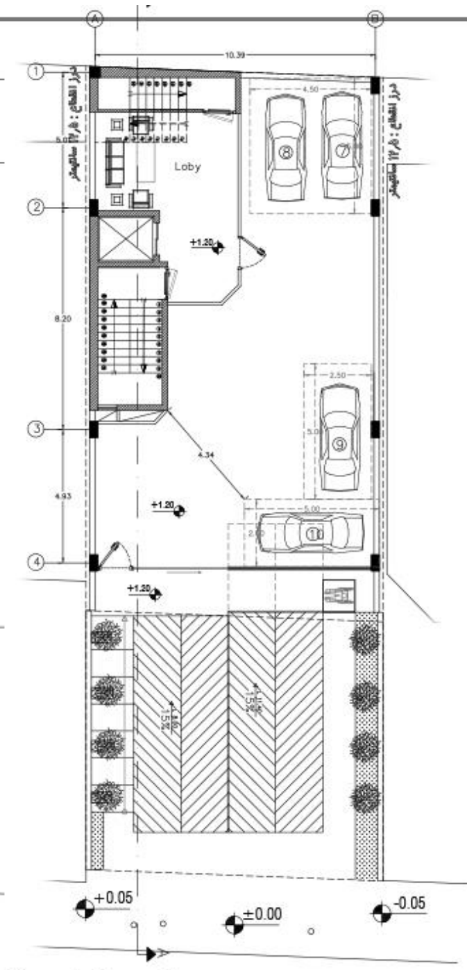
Ground Floor Plane
