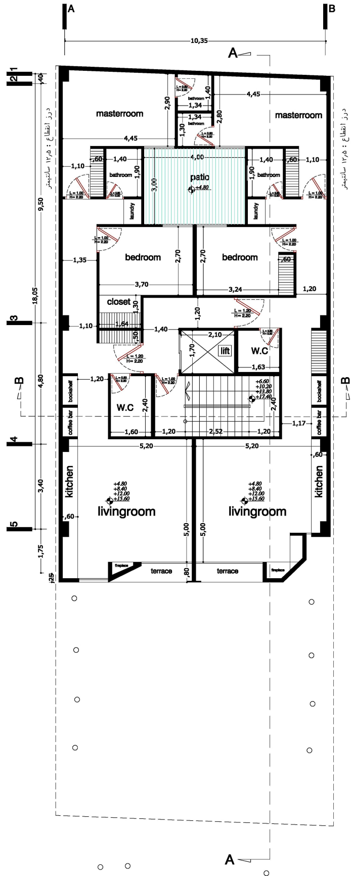
1 & 3 & 5 FLOOR
