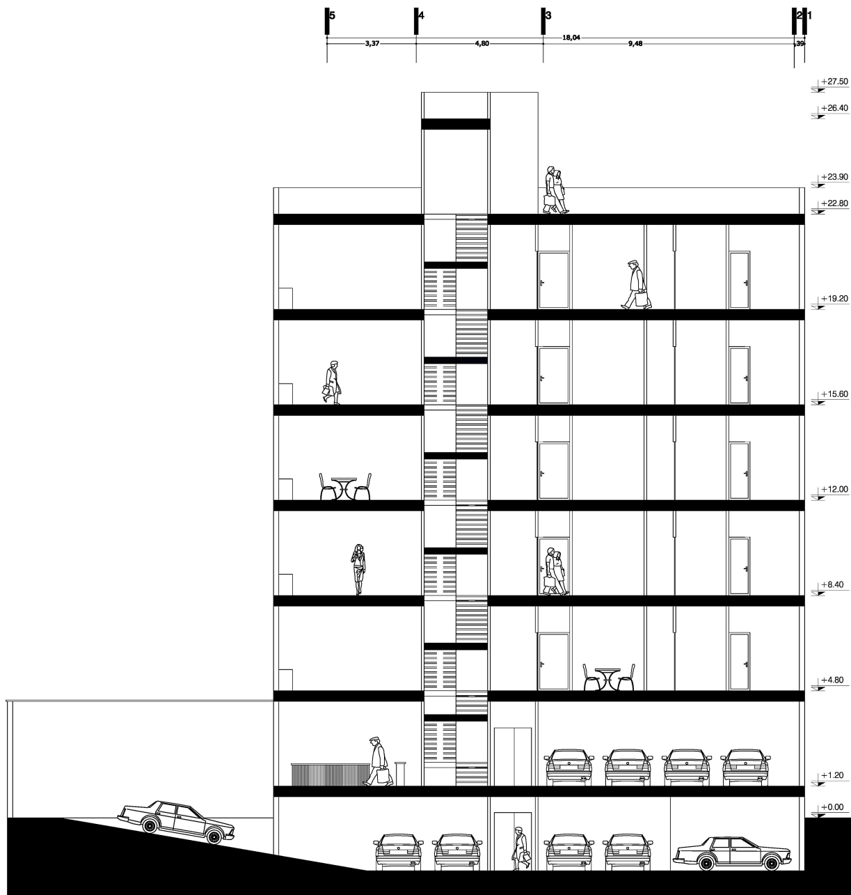
SECTION
