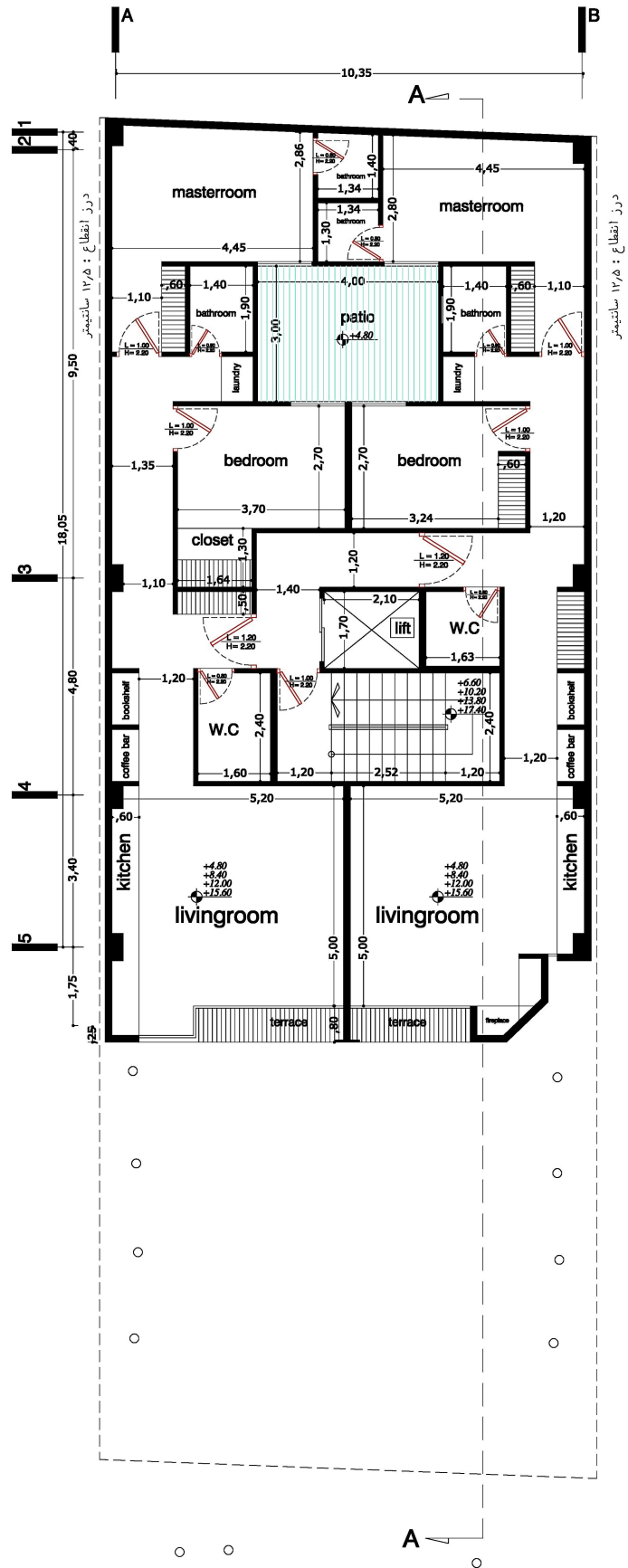
2 & 4 FLOOR
