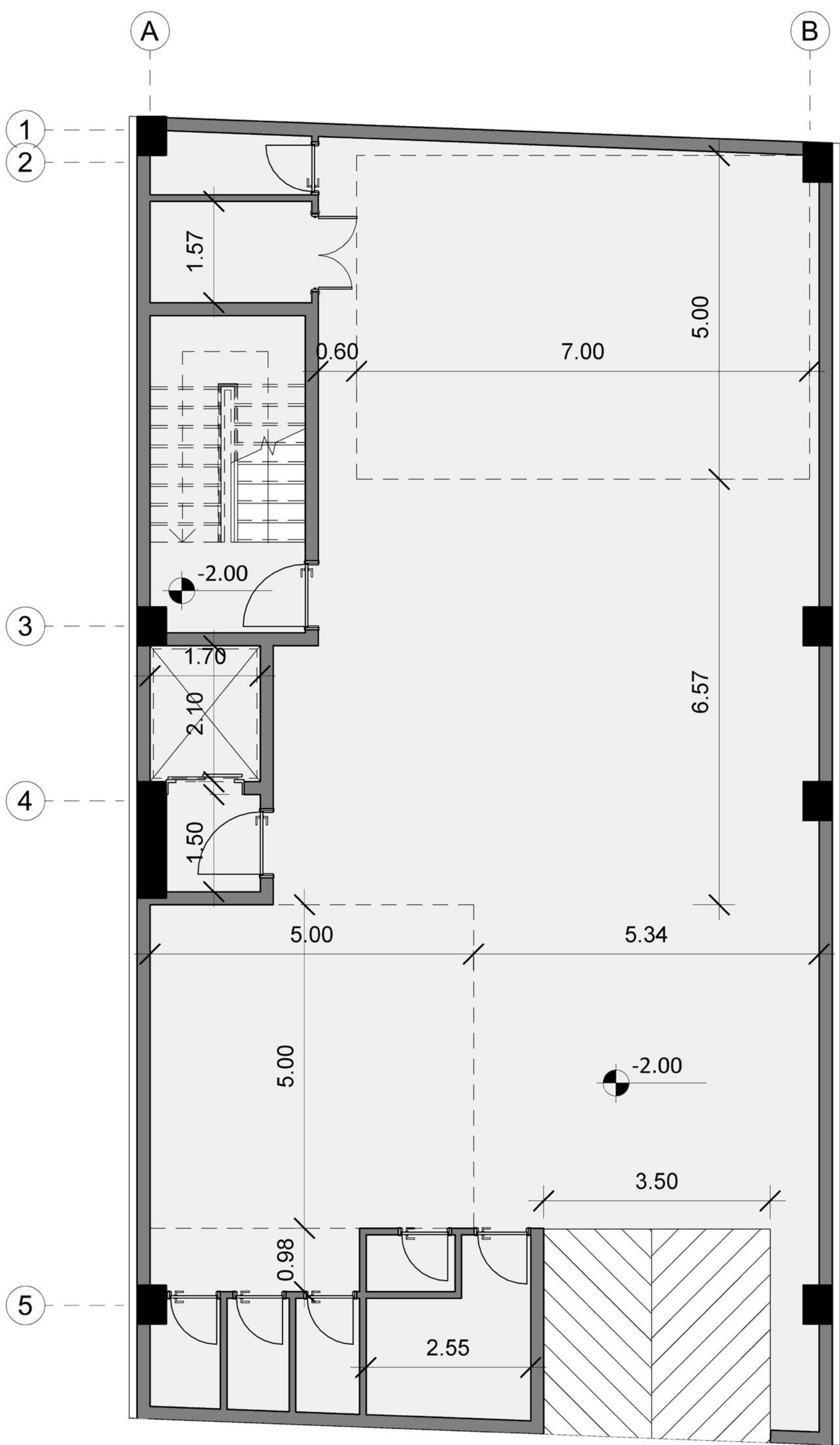
BASEMENT FLOOR DIMENSION PLAN -2.00
