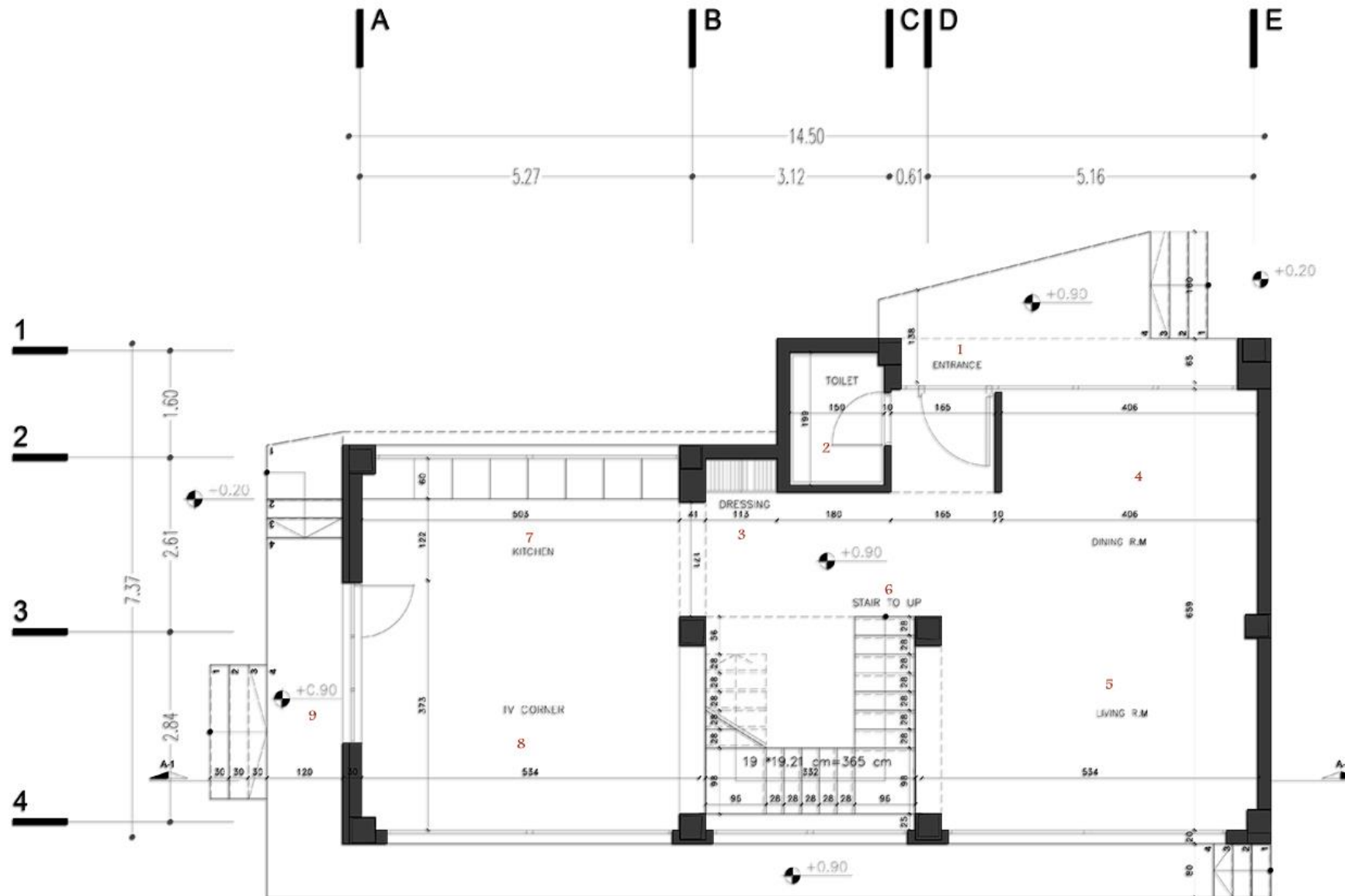
GROUND FLOOR PLAN | SC 1/100
