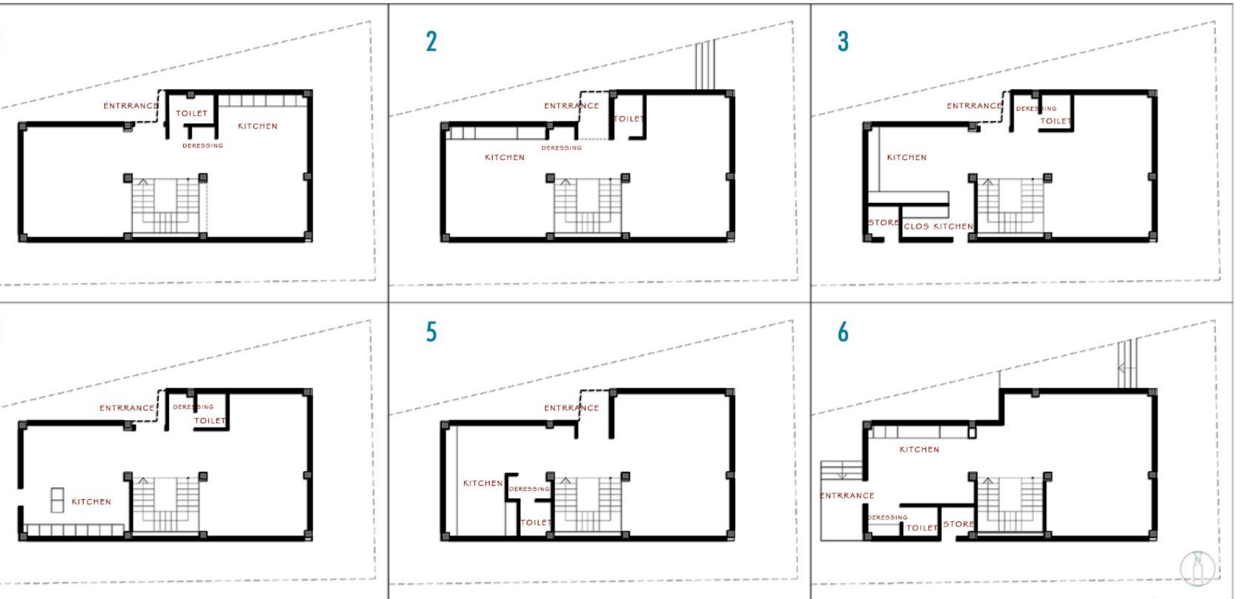
ALTERNATIVE GROUND FLOOR PLAN | SC 1/100
