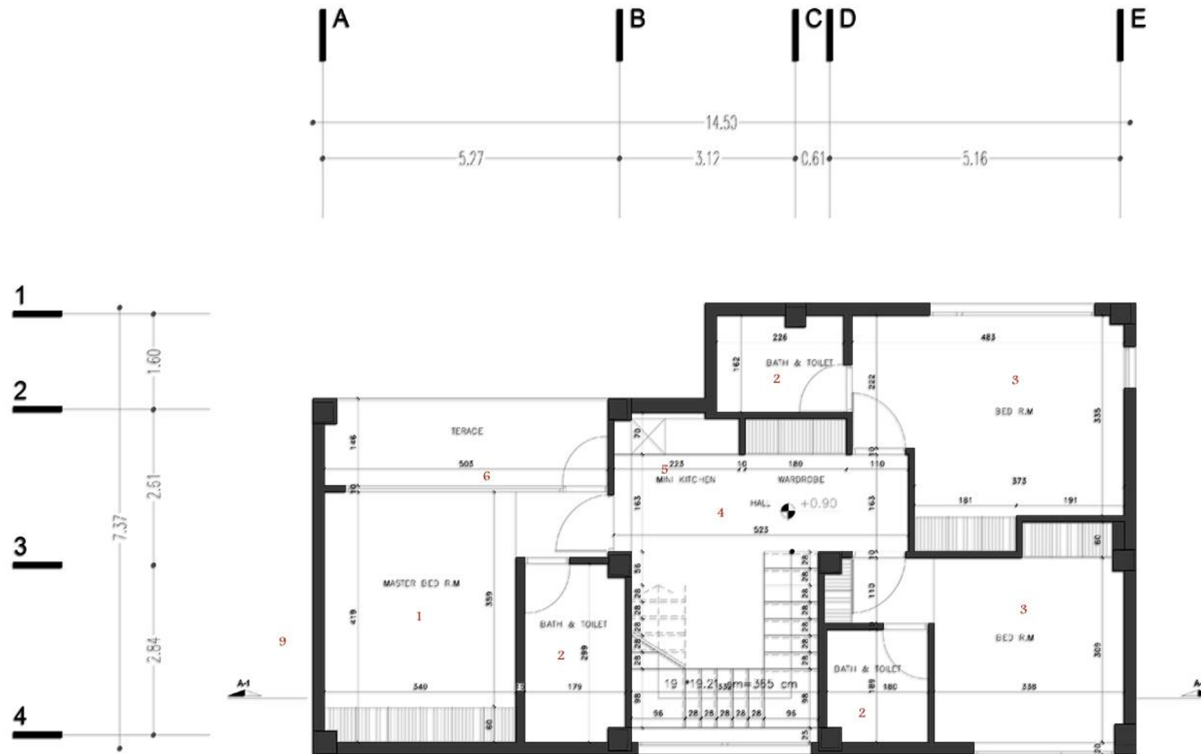
FIRST FLOOR PLAN | SC 1/100
