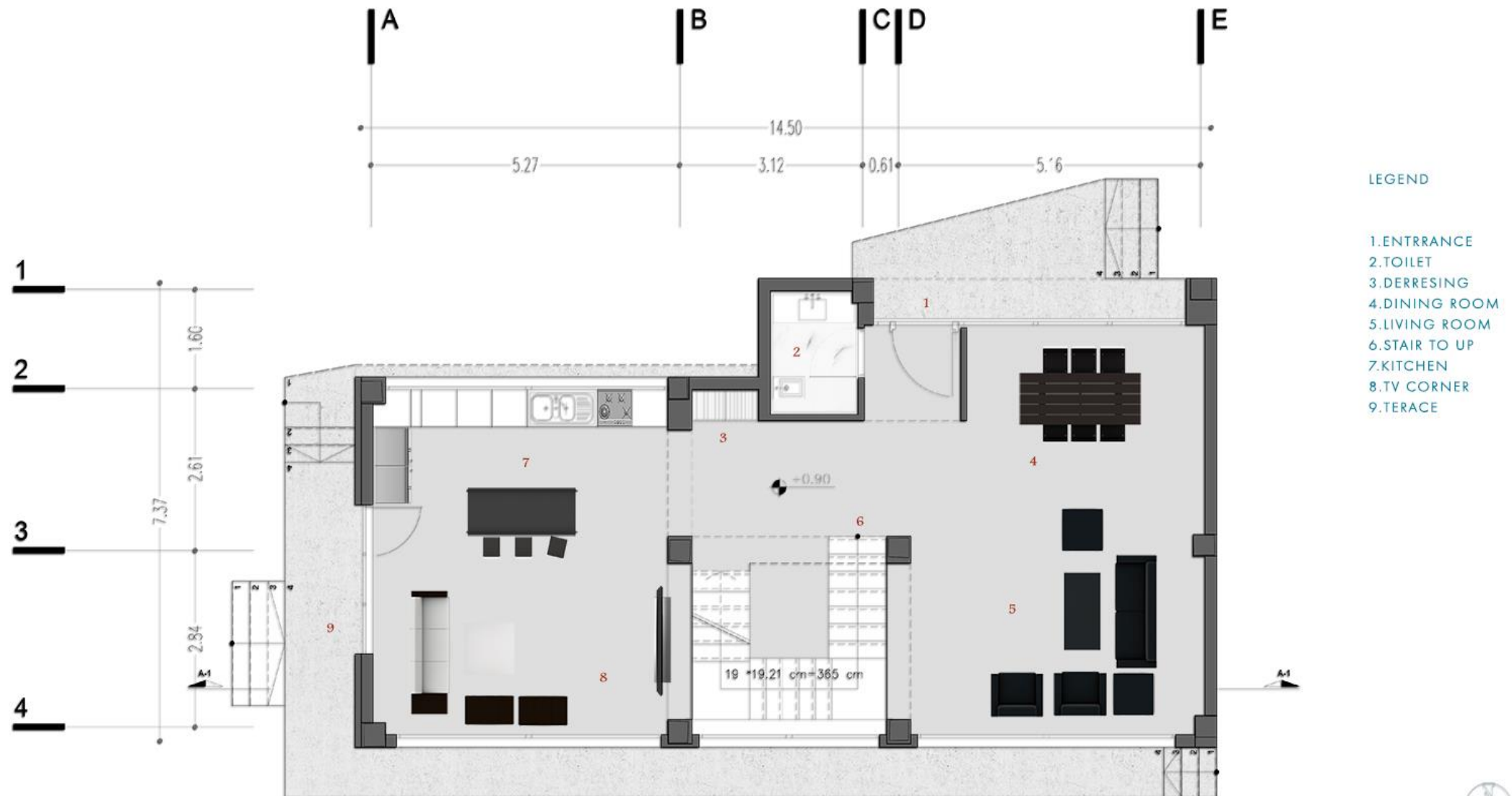
GROUND FLOOR PLAN | SC 1/100
