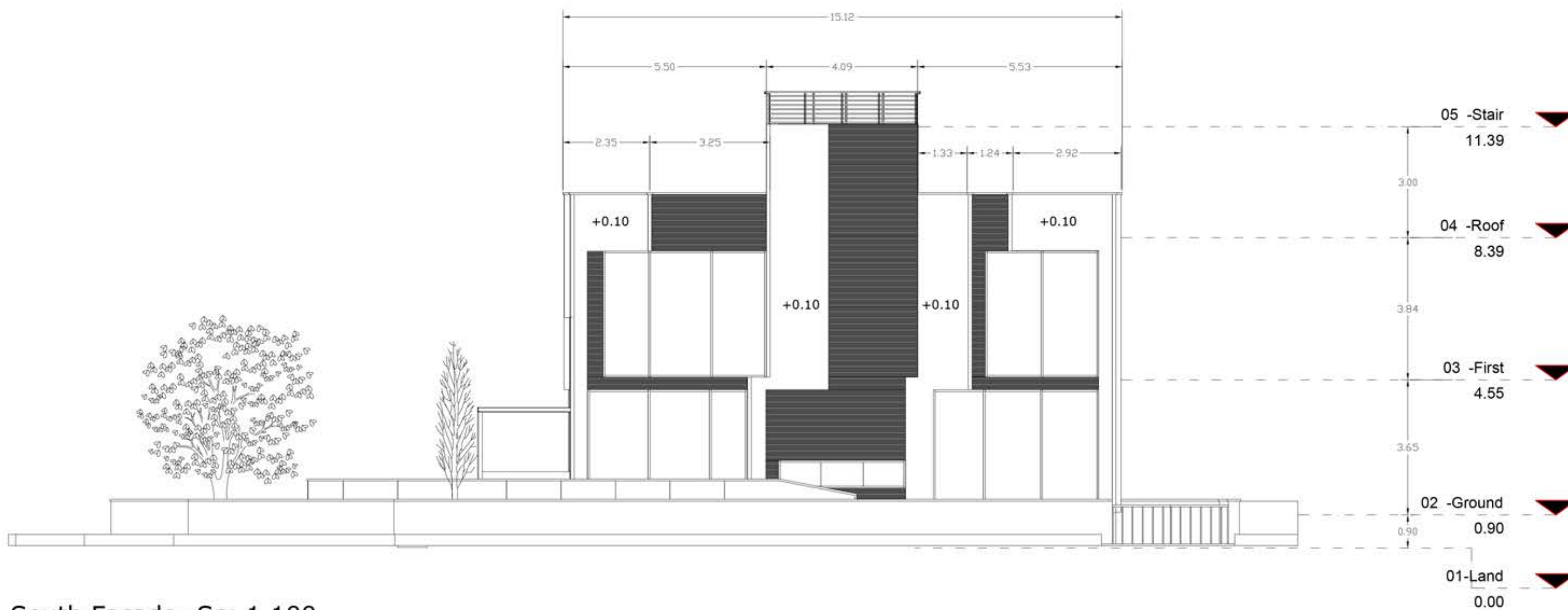
South Facade -Sc: 1.100
