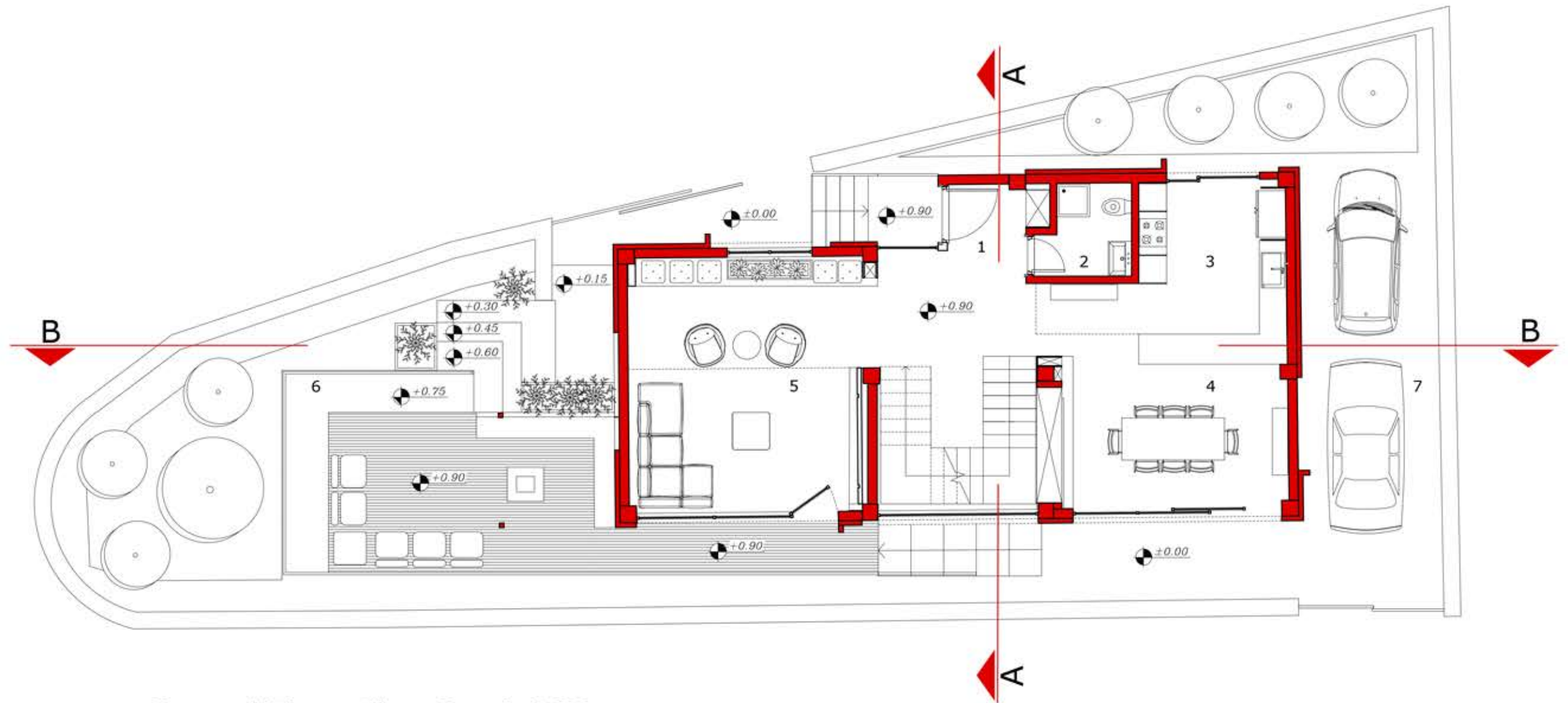
Ground Floor Plan-Sc: 1.100
