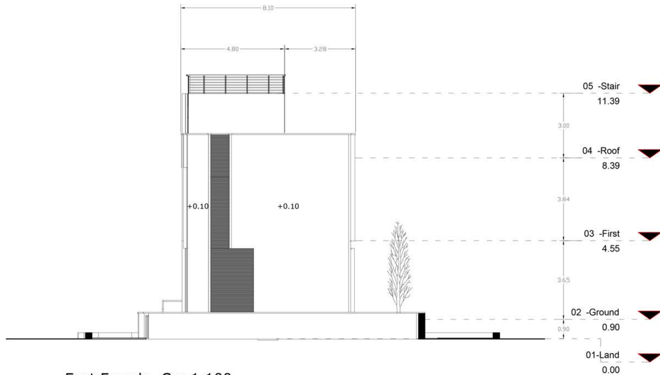
East Facade -Sc: 1.100
