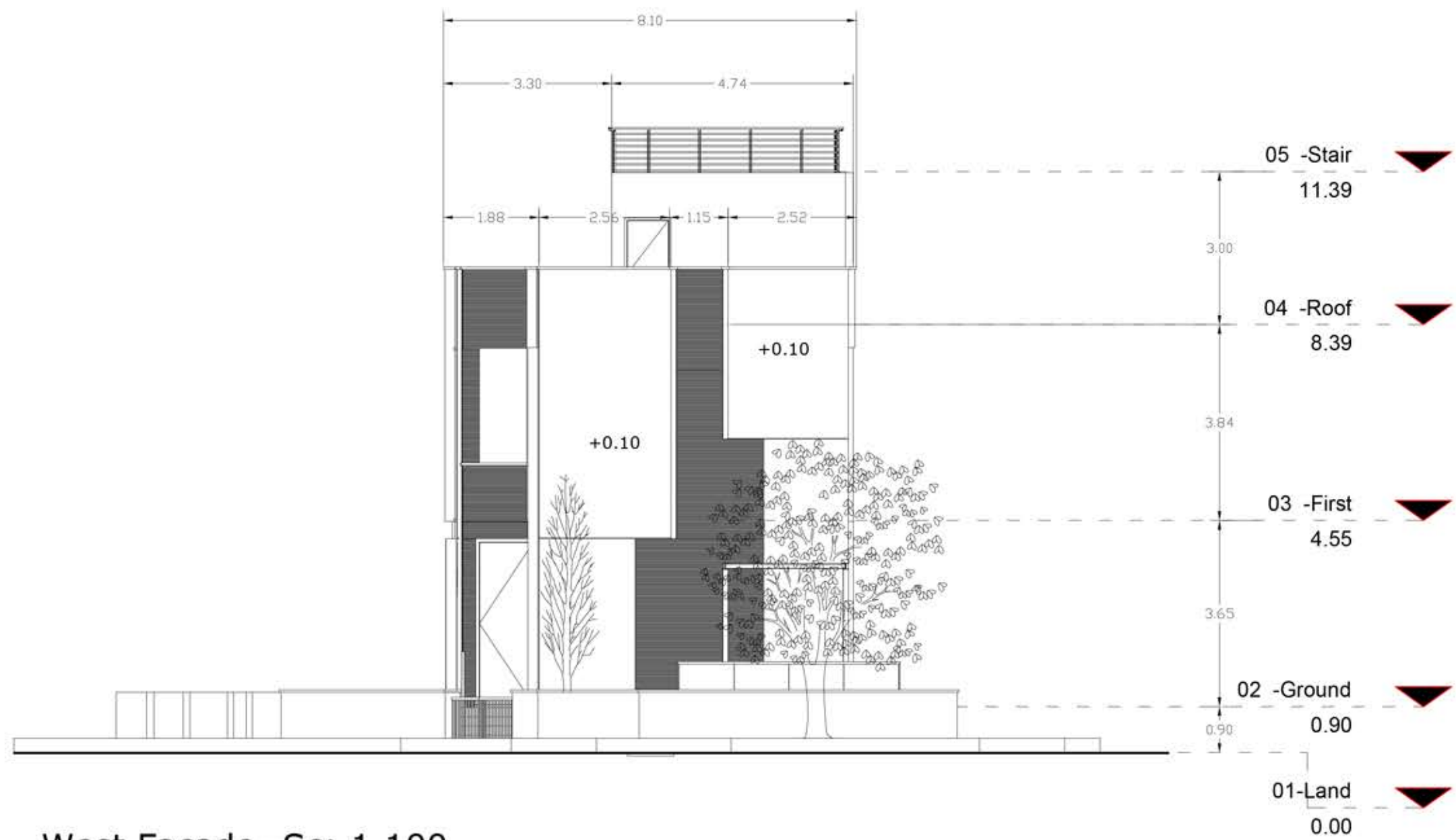
West Facade -Sc: 1.100
