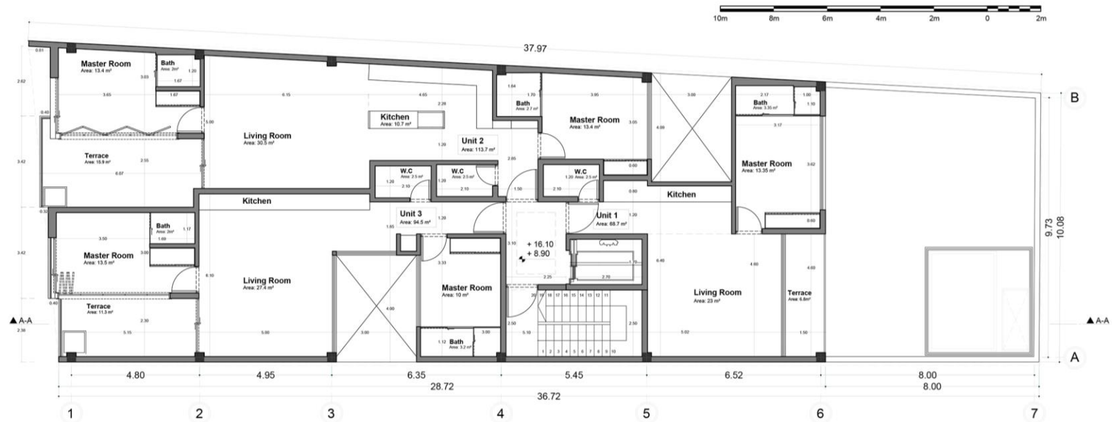
2th 4th Floor Plan
