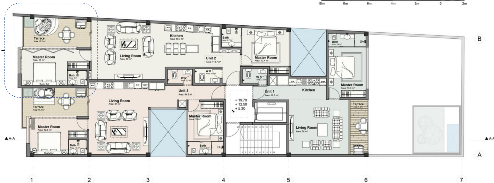
1th 3th 5th Floor Plan
