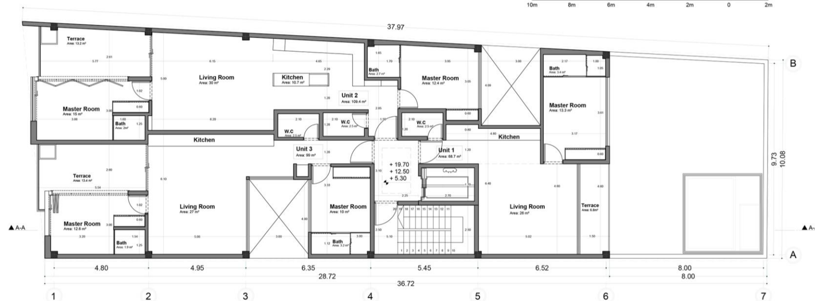
1th 3th 5th Floor Plan
