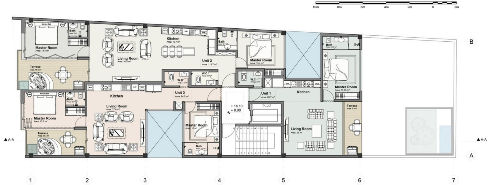
2th 4th Floor Plan
