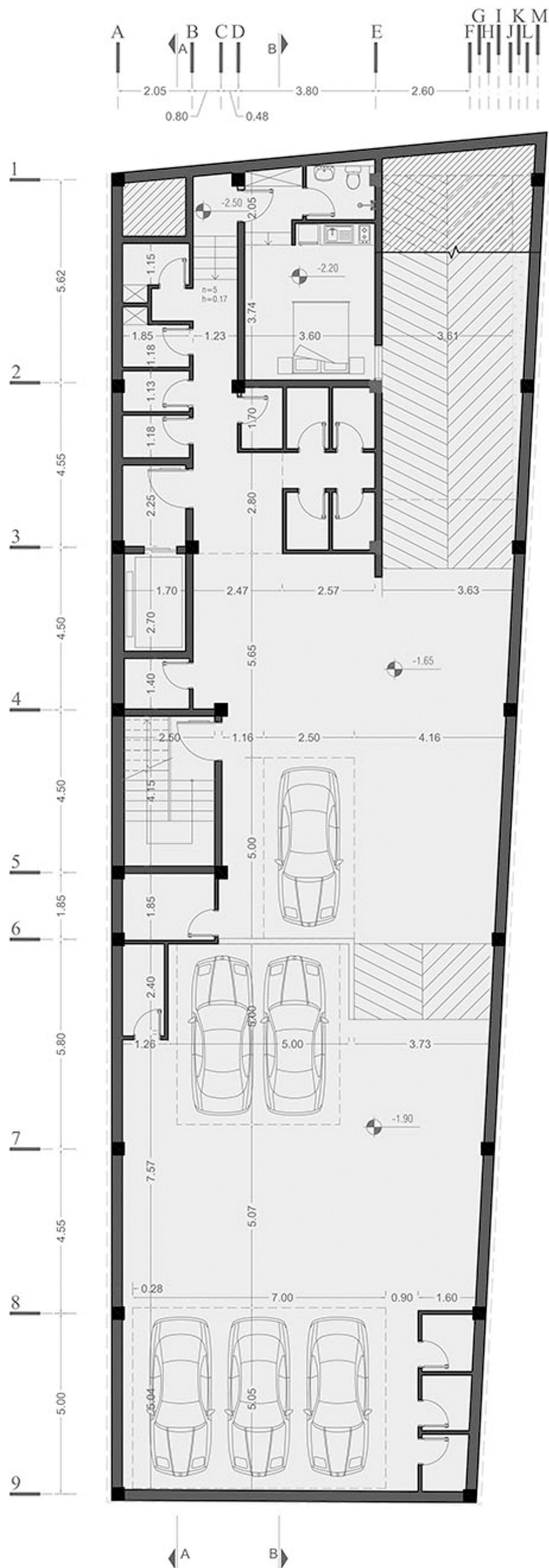
Basement Dimensions Plan
