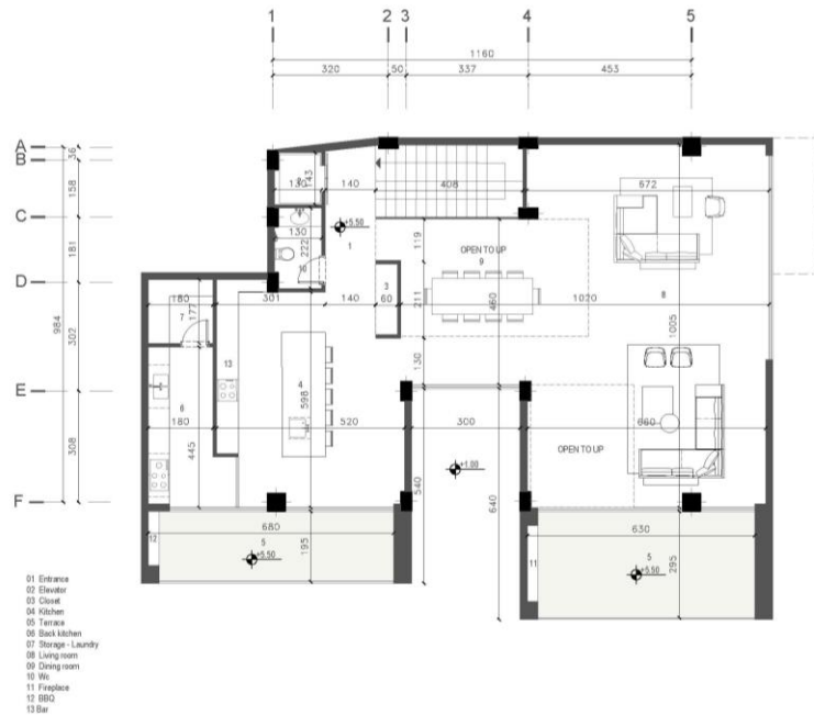
LEVEL 01 DIMENTION PLAN
