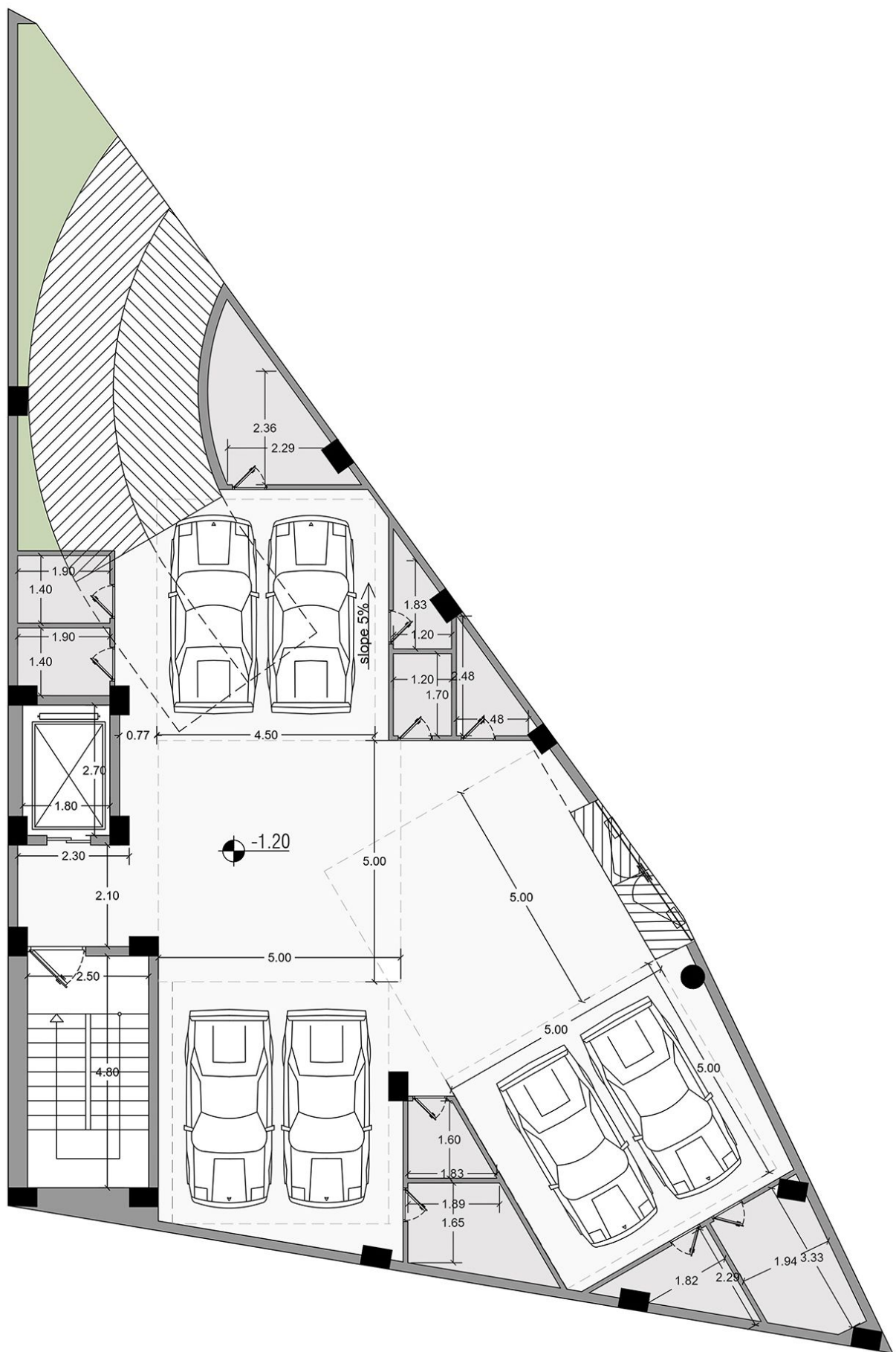
Basement 1
