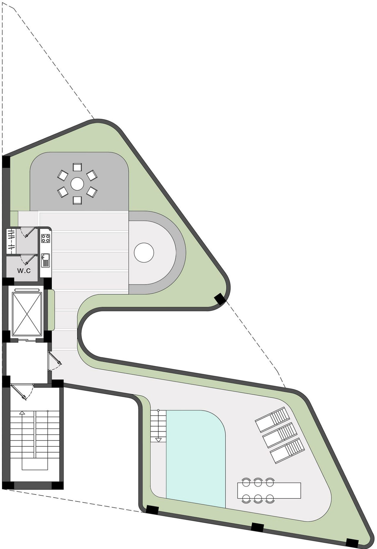
Roof
