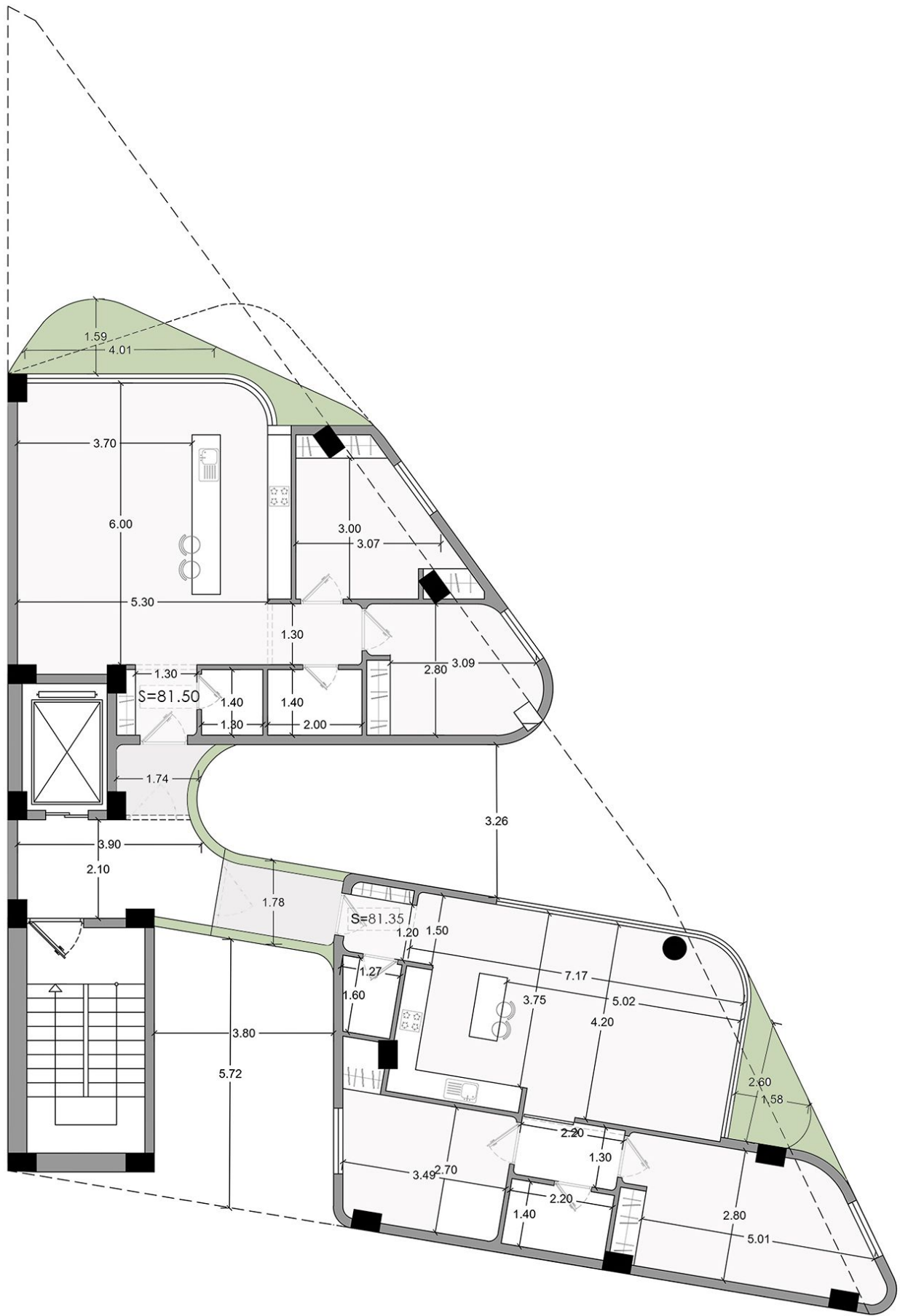
Floor Plan
