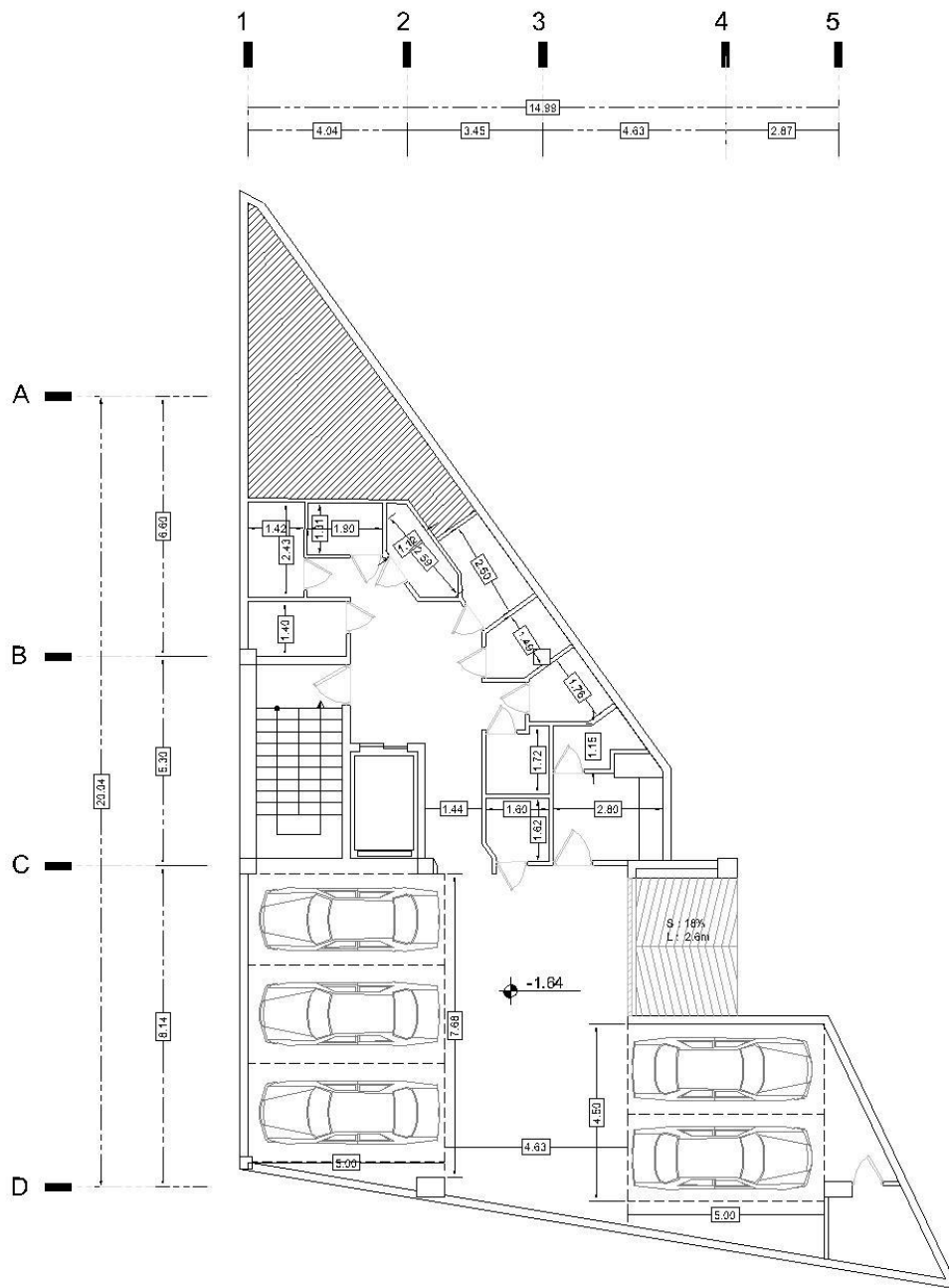
Floor -1
