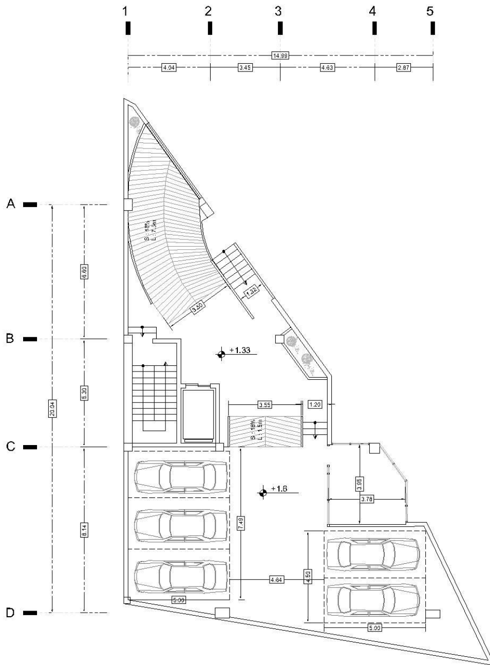
Floor 0
