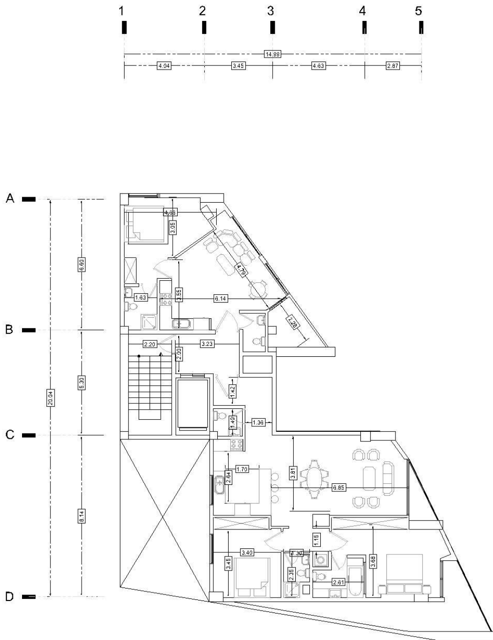
4th floor
