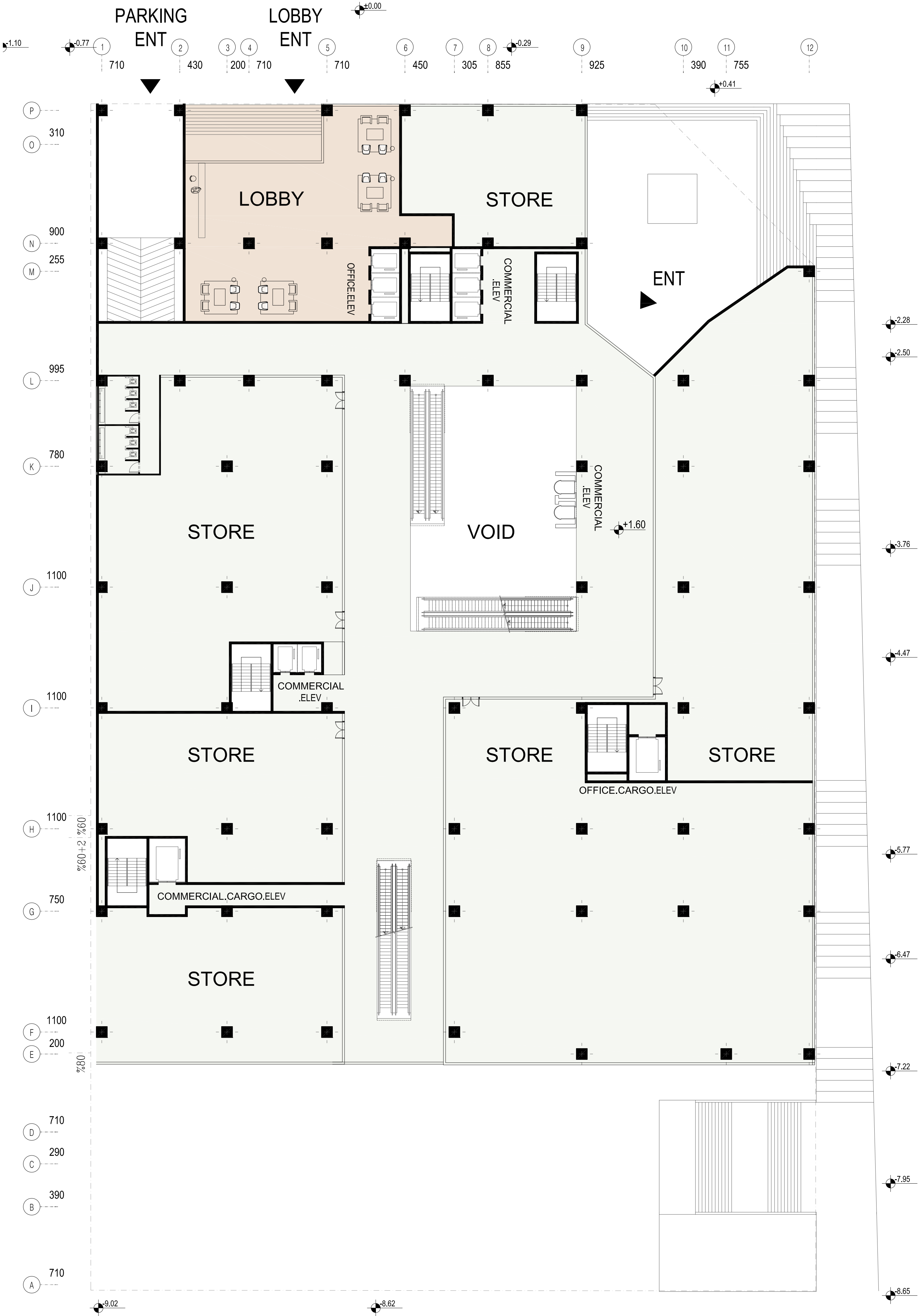
1 2 5 10 20 GROUND FLOOR PLAN TOTAL AREA | 4750 M2
