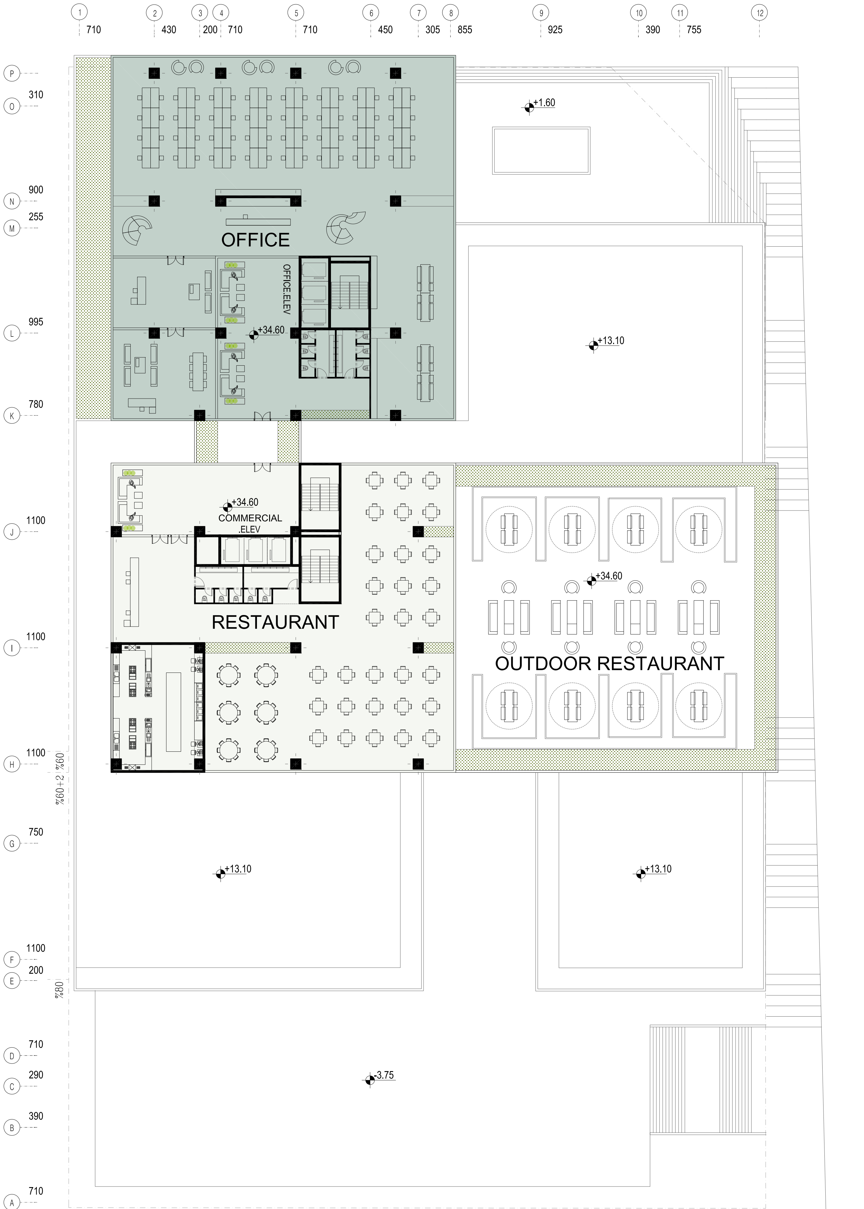
6TH FLOOR PLAN TOTAL AREA | 2085 M2
