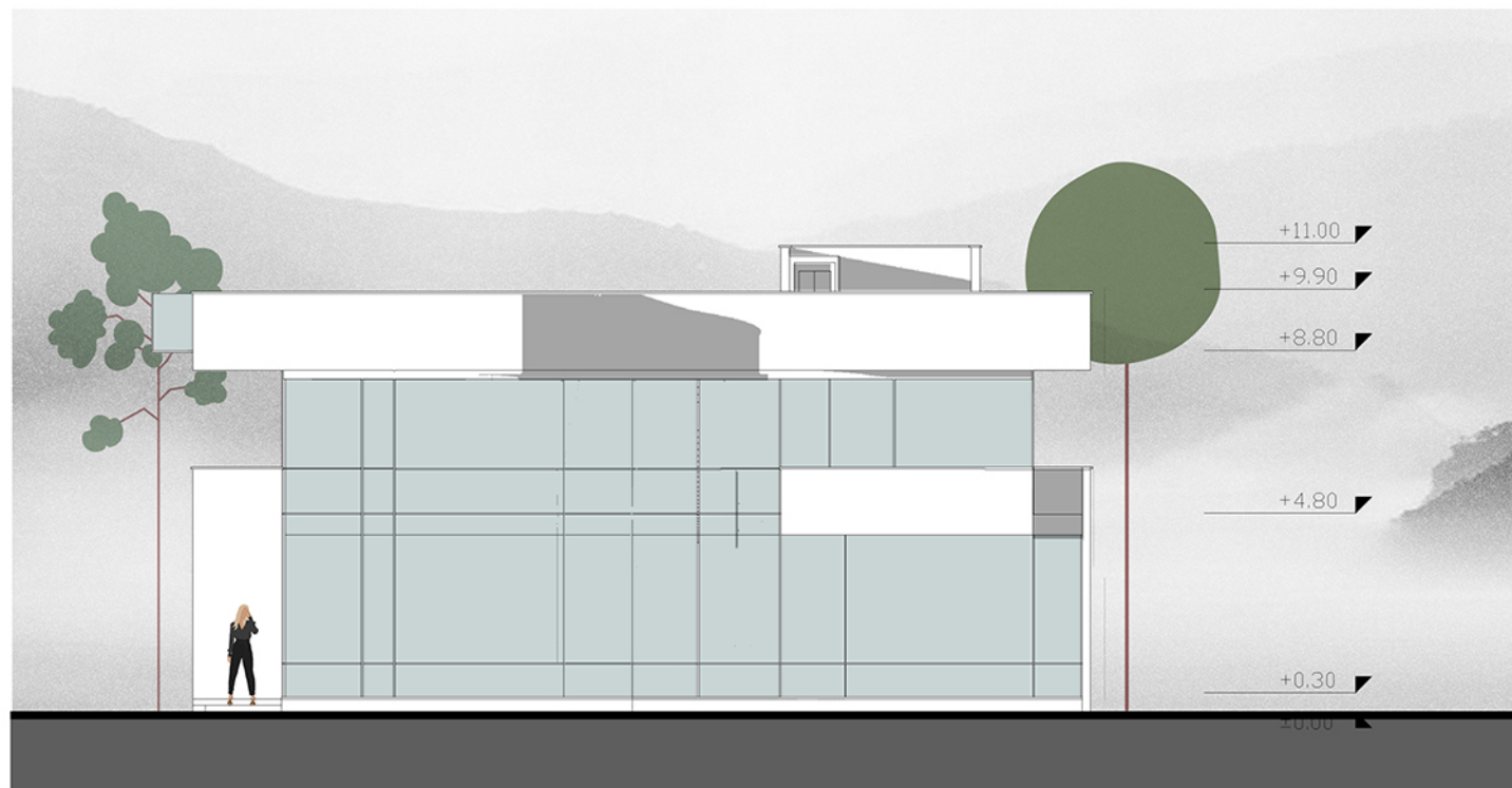
NORTH ELV
