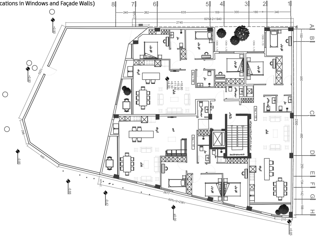
Fifth Floor Plan (Modifications in Windows and Façade Walls)
