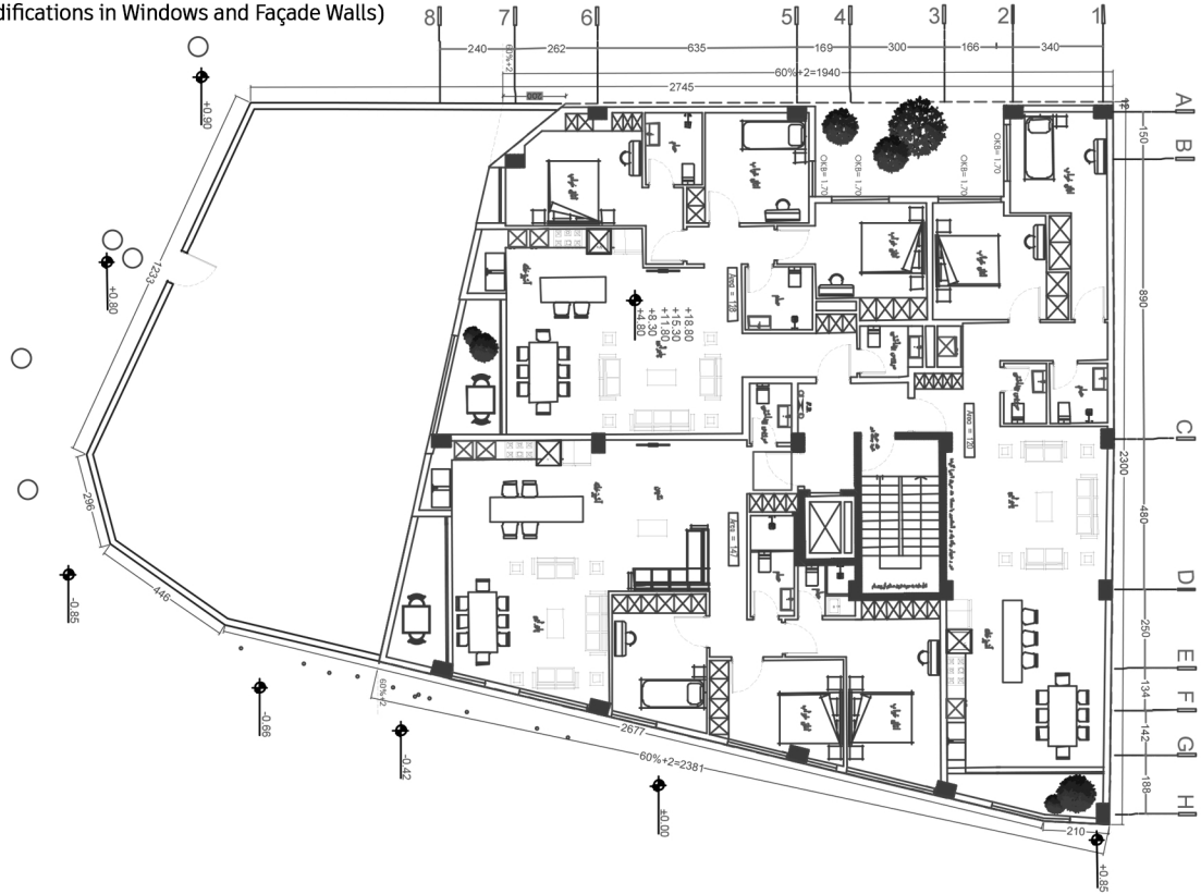
Second Floor Plan (Modifications in Windows and Faade Walls)
