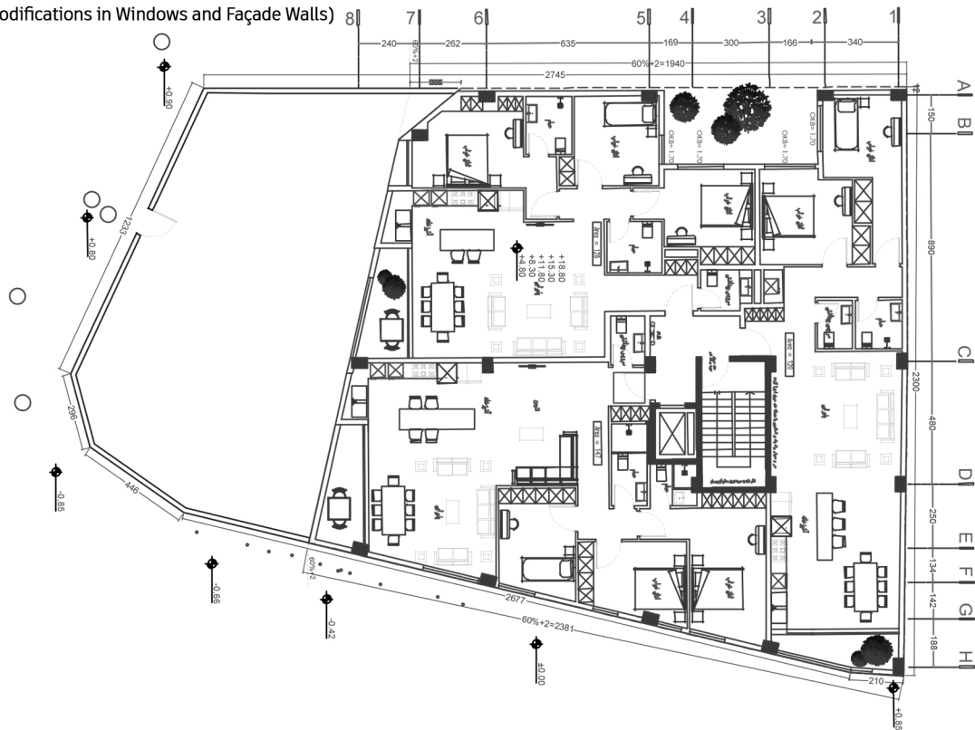
First Floor Plan (Modifications in Windows and Façade Walls)
