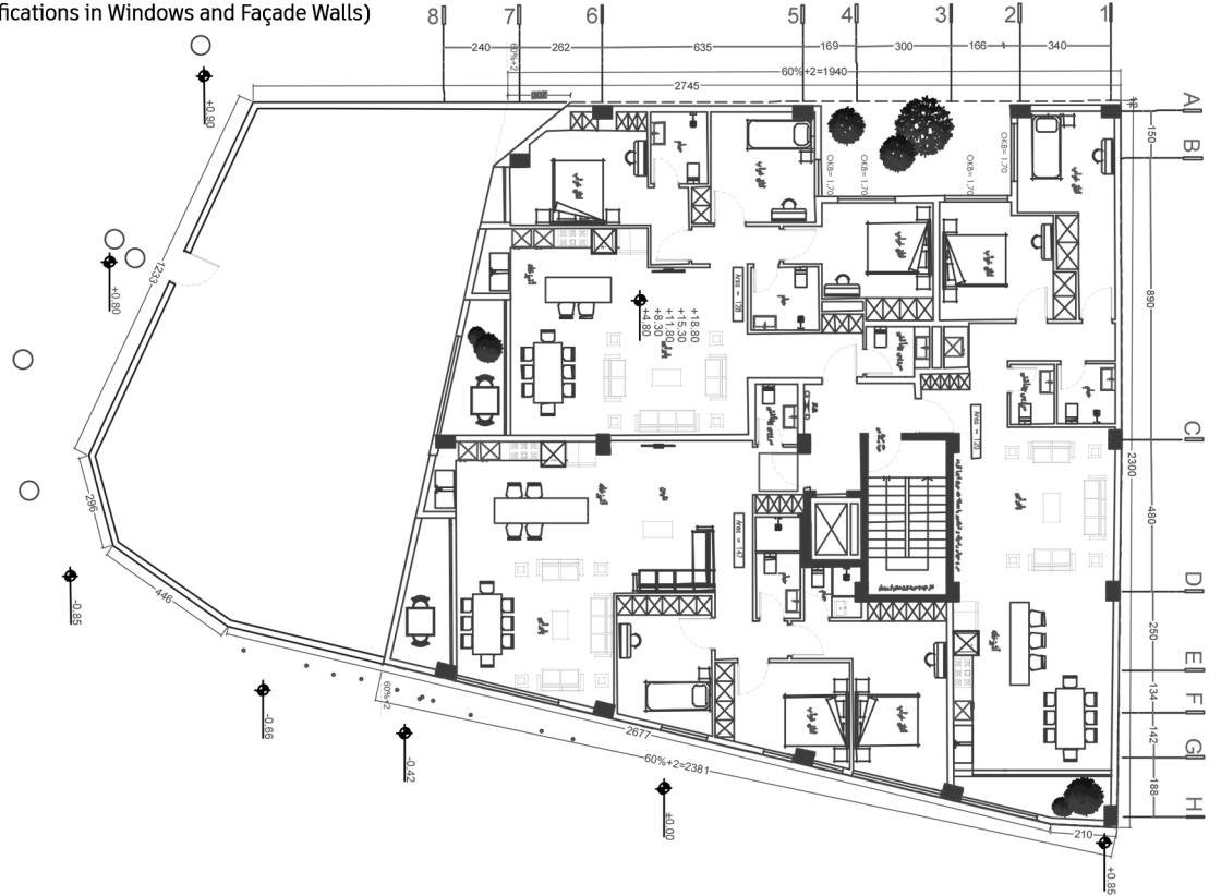
Third Floor Plan (Modifications in Windows and Faade Walls)
