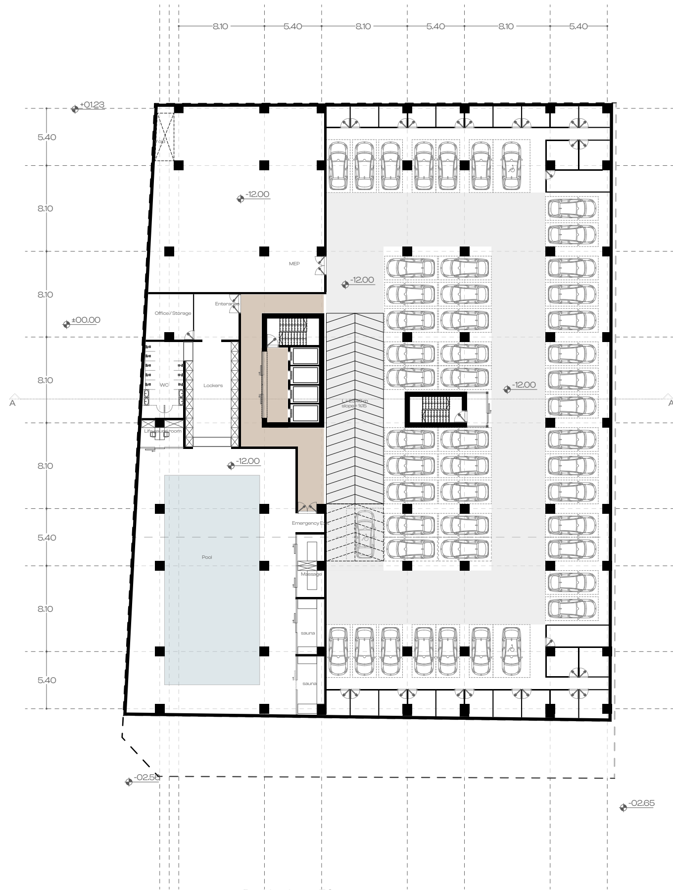
-4th Basement Floor Plan
