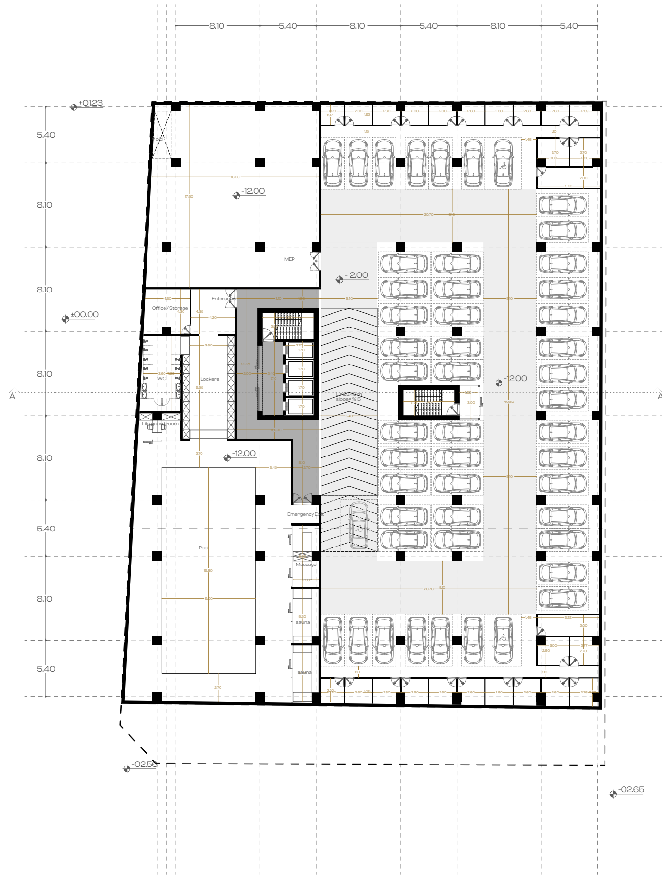
-4th Basement Floor Plan | Parking lots = 50 Level = -12.00
