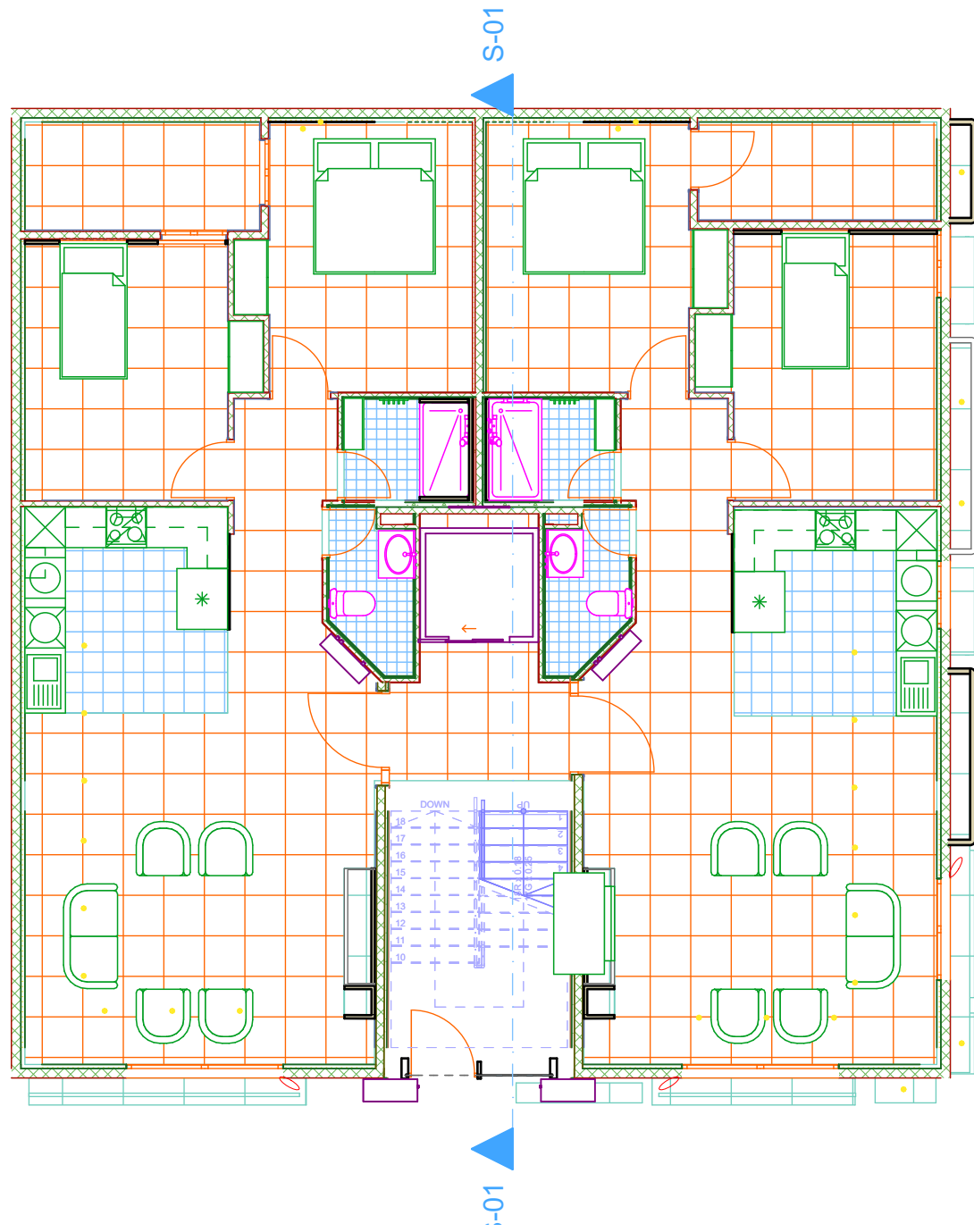
1. Story 1:100
