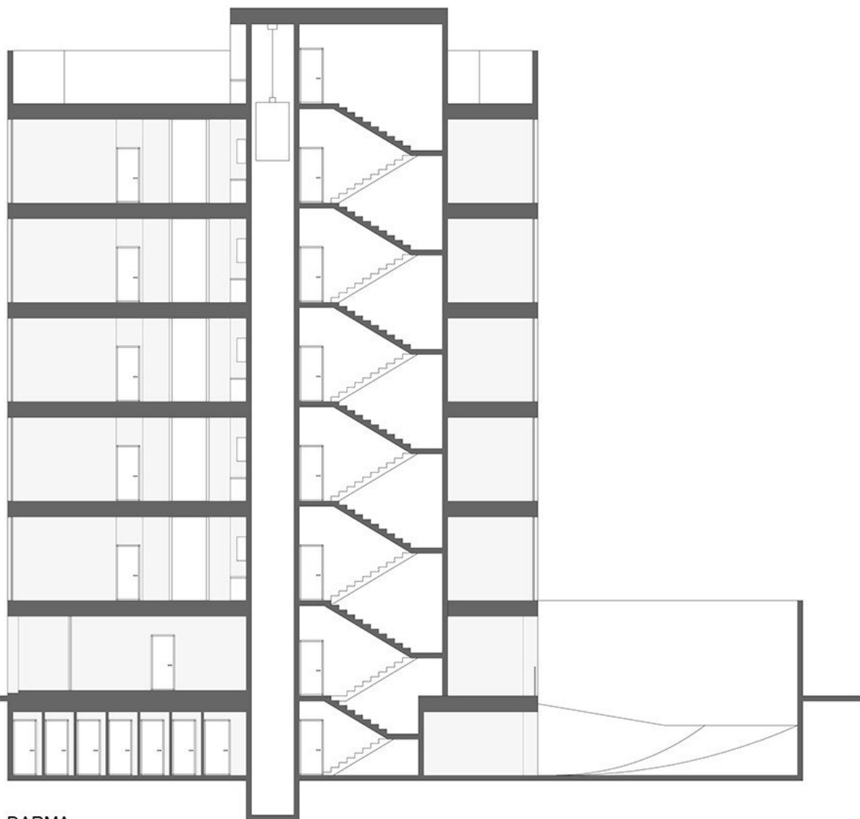
DARMA apartment section A-A
