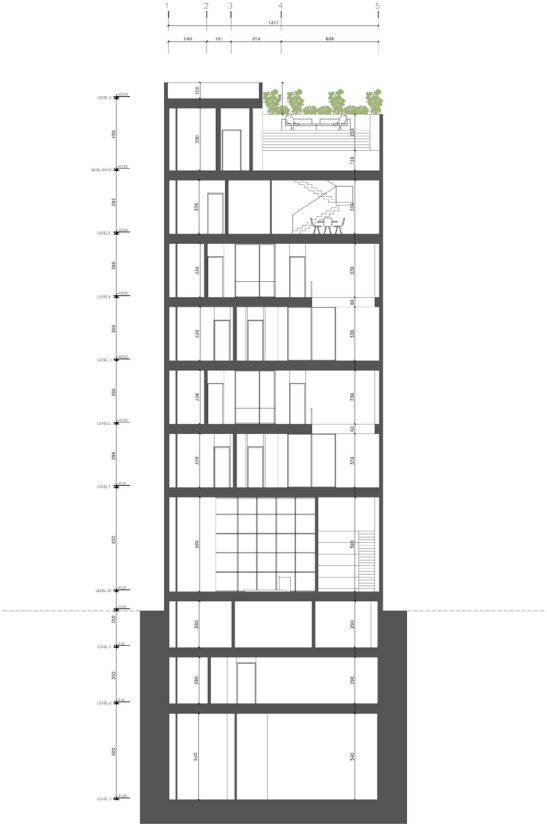
NARENJESTAN RESIDENCE SECTION A-A
