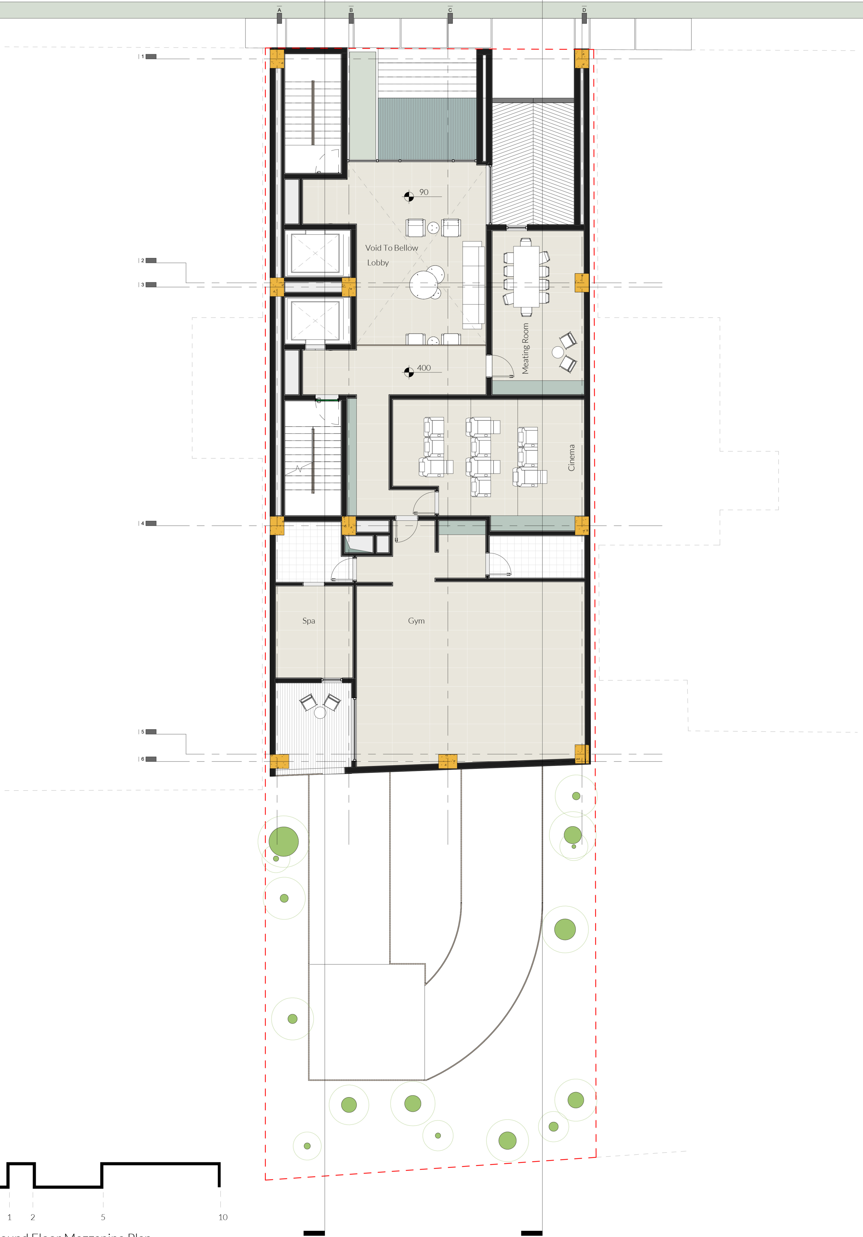
Ground Floor Mezzanine Plan
