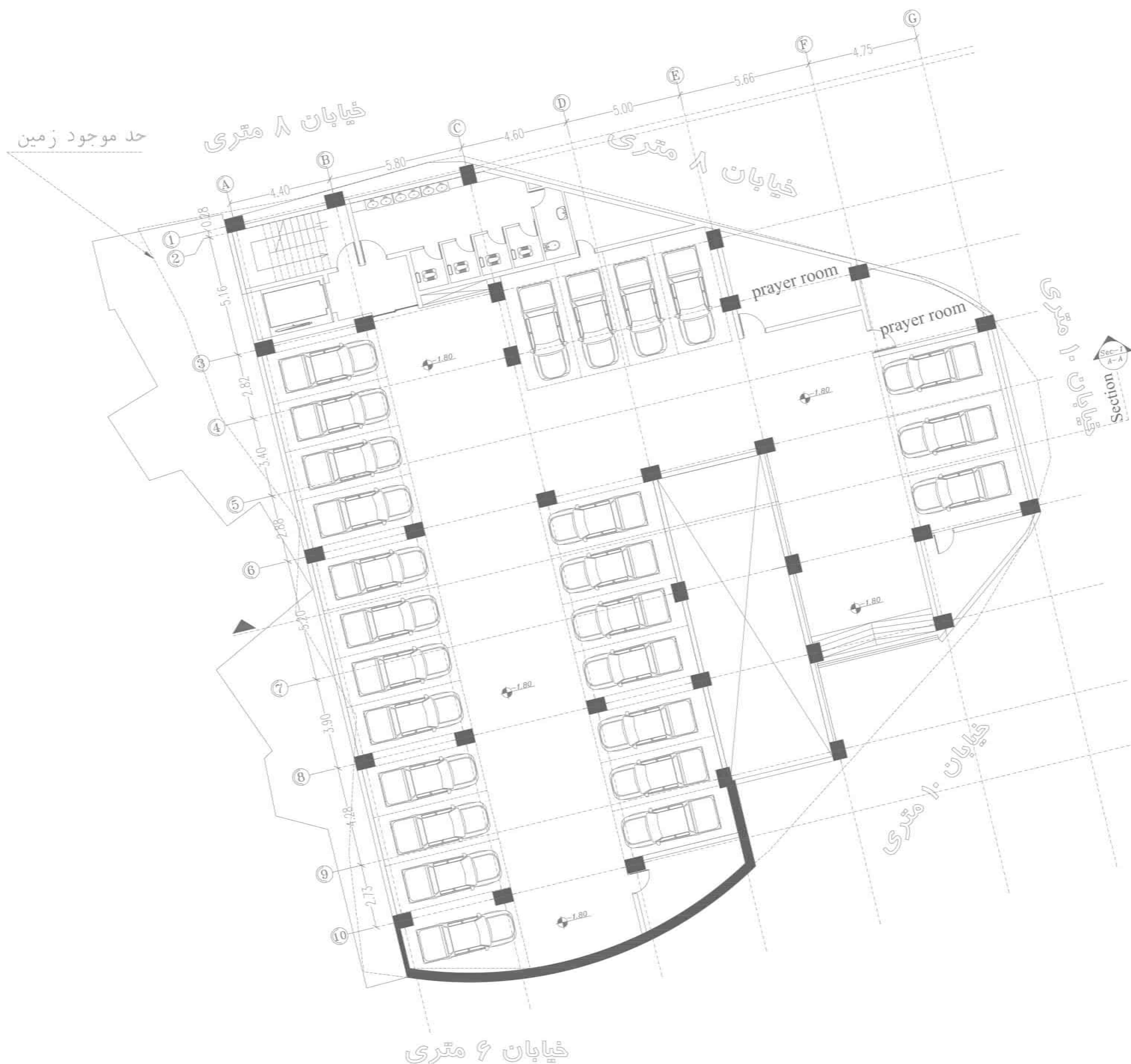
First basement floor Scale. 1:100 furniture plan
