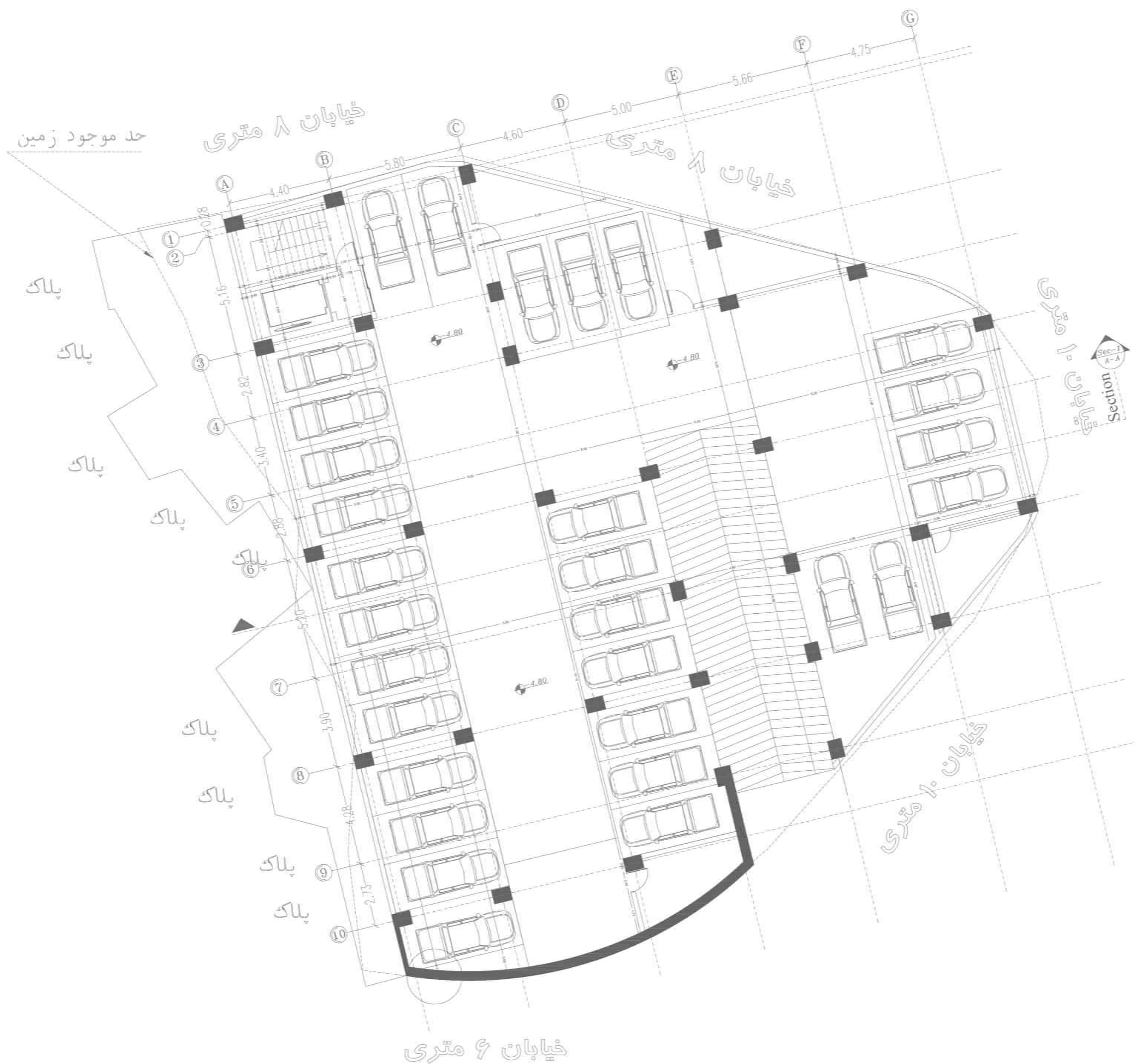
Second basement floor Scale. 1:100 Measurement plan
