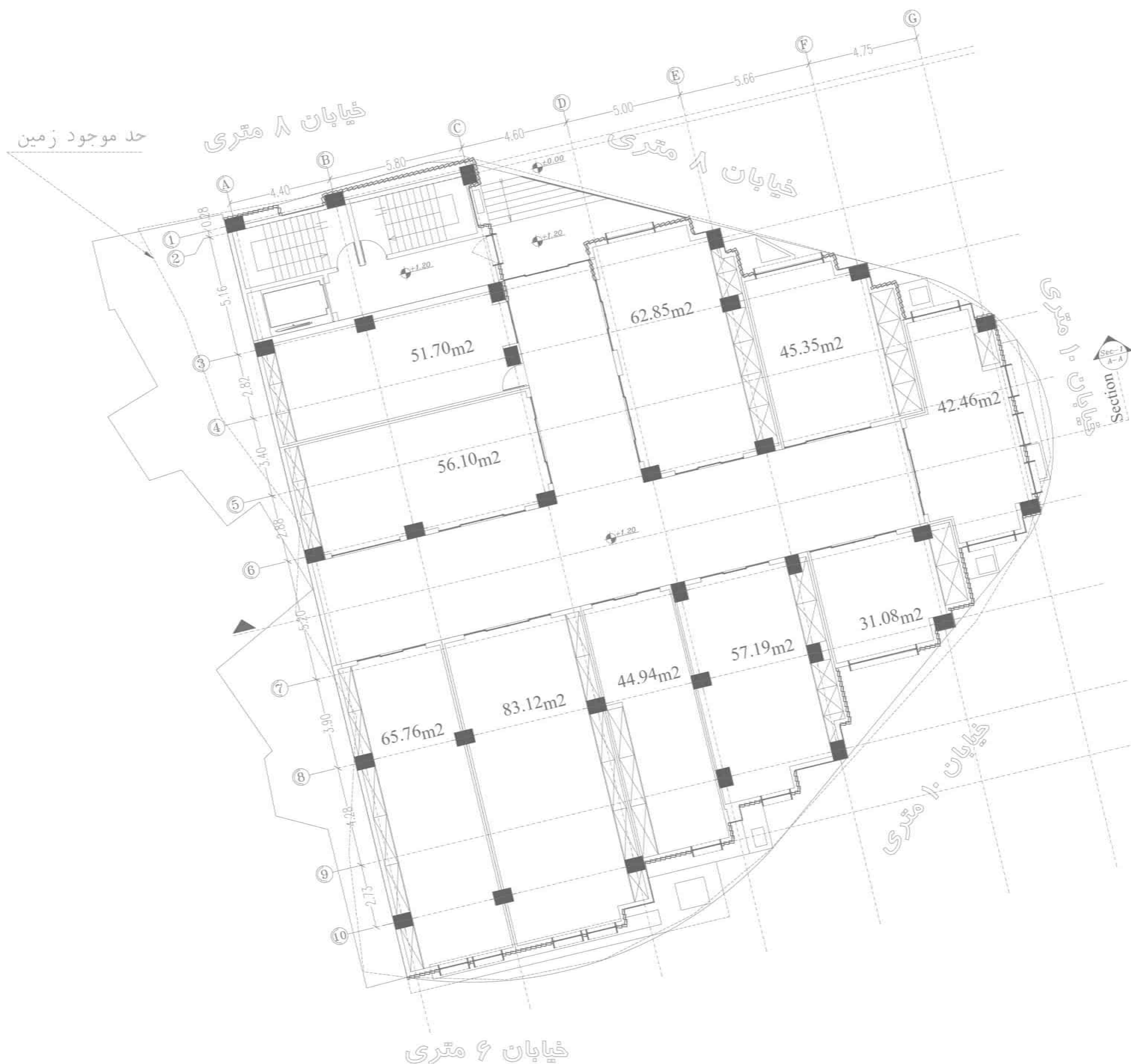
Ground floor plan Scale: 1:100 furniture plan
