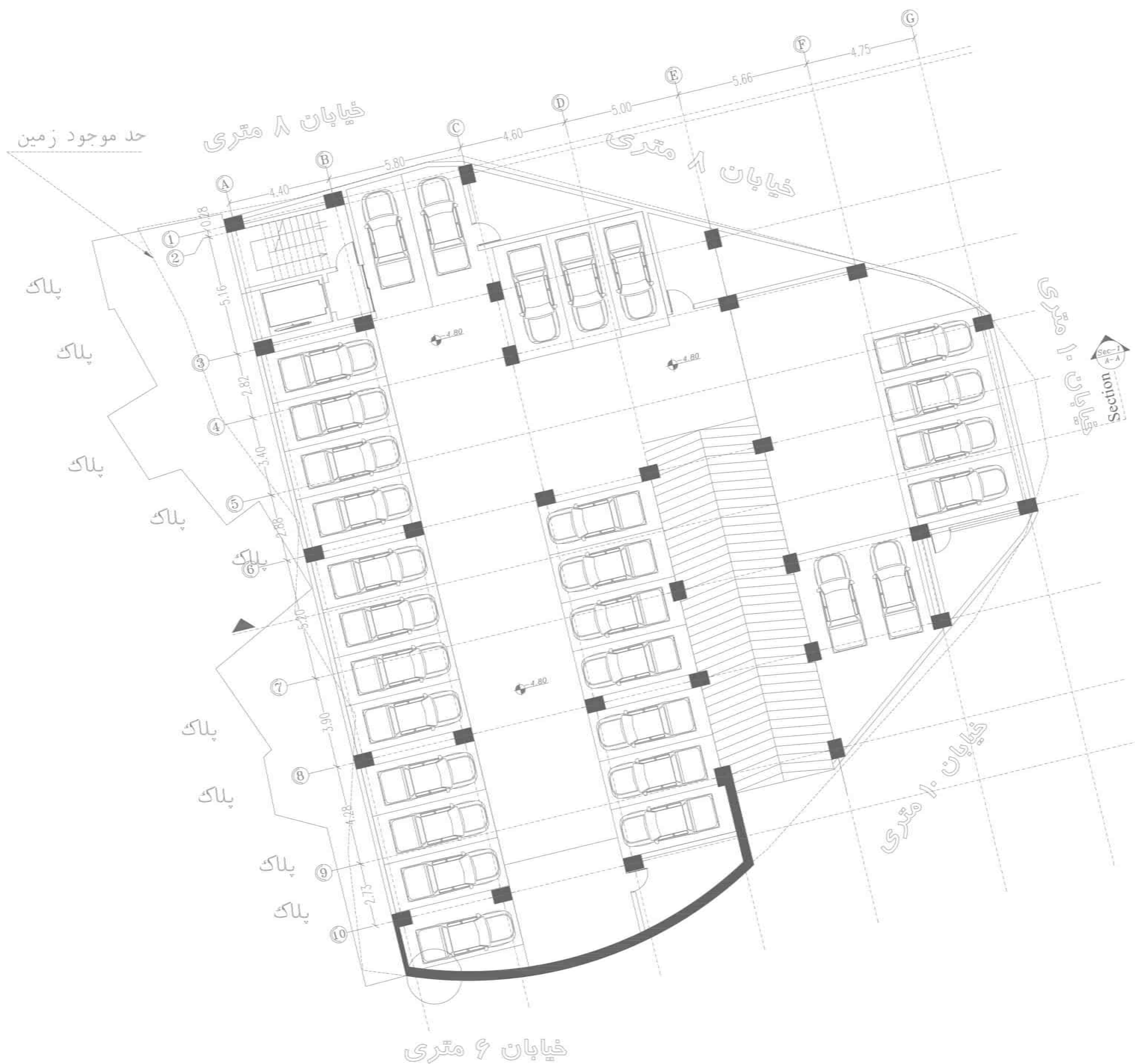
Second parking floor Scale. 1:100 furniture plan
