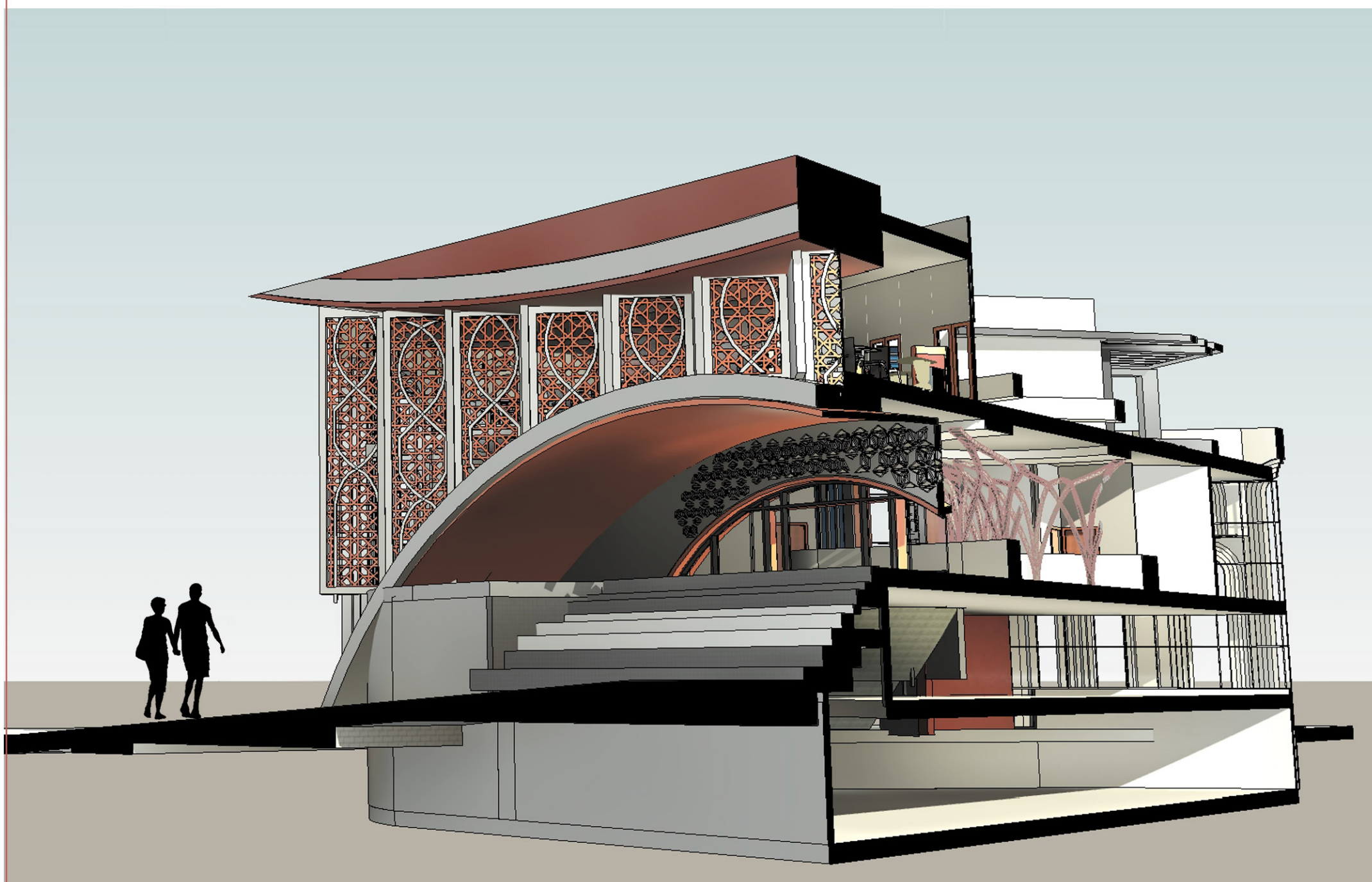
SECTION & PERSPECTIVE
