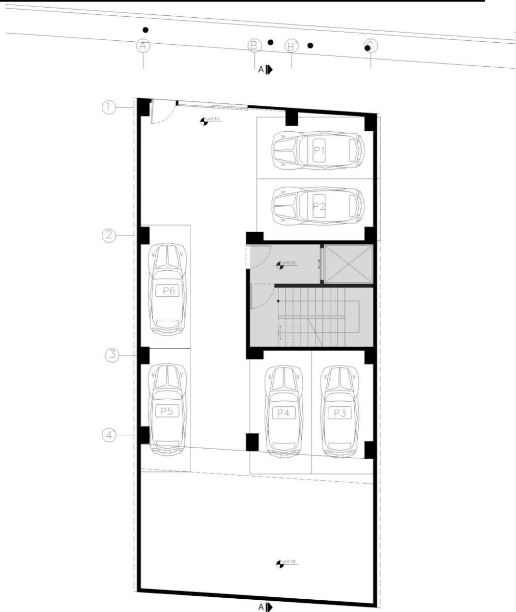
GROUND FLOOR
