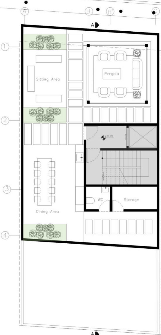
ROOF GARDEN
